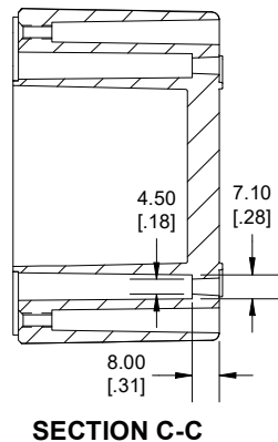
SECTION C-C
