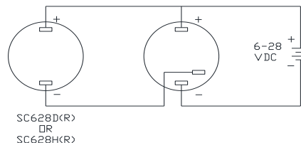
Wiring Diagram
