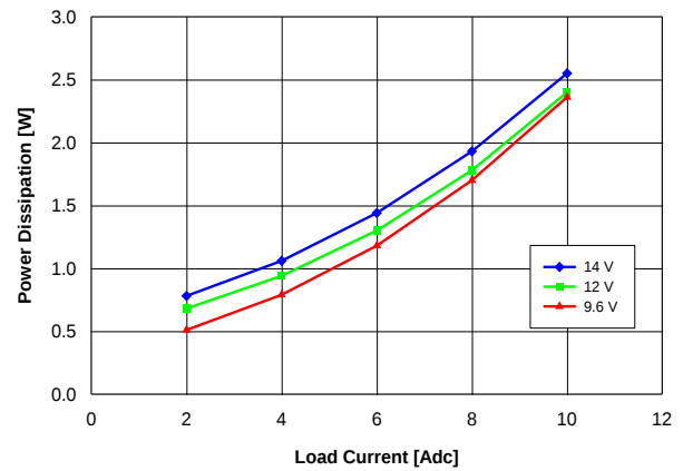
Fig. 2.5V.4: Power Loss vs. load current and input voltage for V_{out} = 2.5V converter mounted vertically with air flowing at a rate of 200 LFM (1 m/s) and T_a = 25^\circ C .
