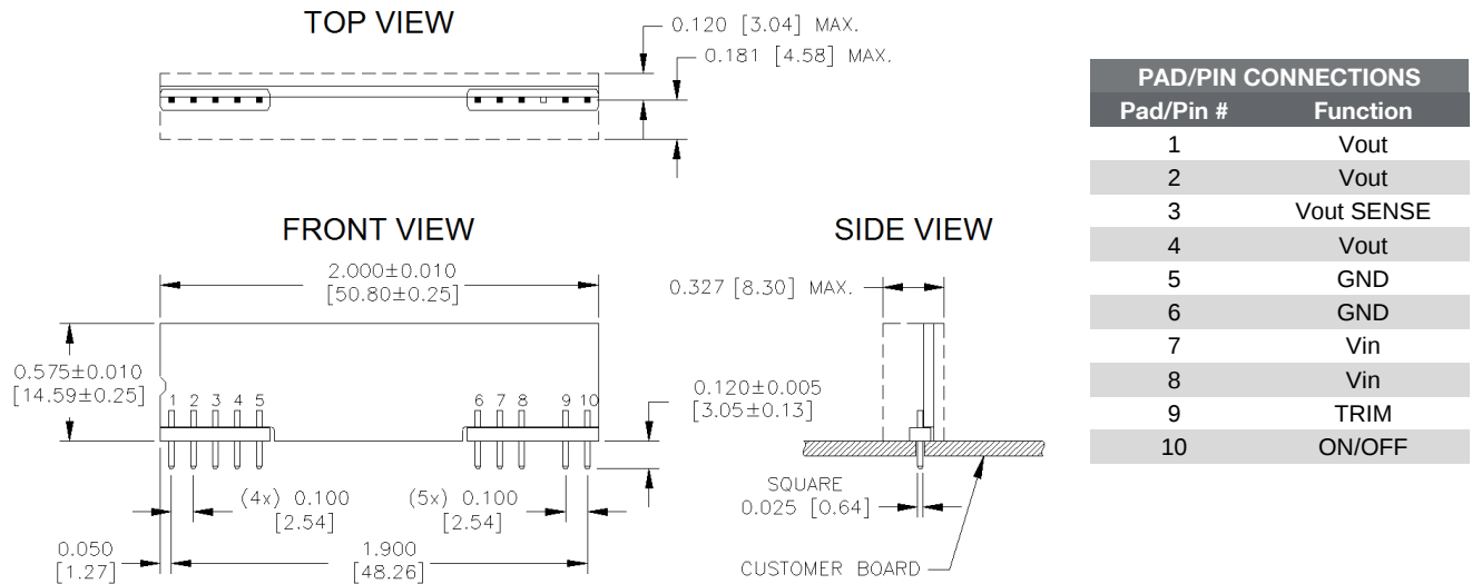
YNV12T10 Pinout (Through-Hole - SIP)
