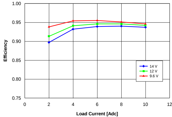
Fig. 5.0V.3: Efficiency vs. load current and input voltage for V_{out} = 5.0V converter mounted vertically with air flowing at a rate of 200 LFM (1 m/s) and T_a = 25^{\circ}C .
