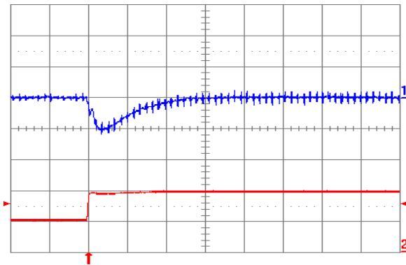
Fig. 1.8V.7: Output voltage response for V_{out} = 1.8V to positive load current step change from 5A to 10A with slew rate of 5A/\mu s at V_{in} = 12V . Top trace: output voltage (100mV/div.); Bottom trace: load current (5A/div.). C_o = 100\mu F ceramic. Time scale: 20\mu s /div.
