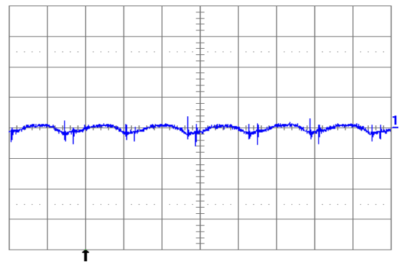
Fig. 1.5V.6: Output voltage ripple (20mV/div.) at full rated load current into a resistive load with external capacitance 100\mu F ceramic and V_{in} = 12V for V_{out} = 1.5V . Time scale: 2\mu s /div.
