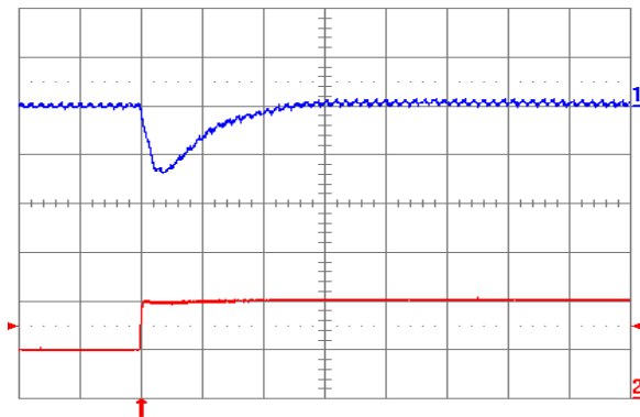
Fig. 2.5V.7: Output voltage response for V_{out} = 2.5V to positive load current step change from 5A to 10A with slew rate of 5A/\mu s at V_{in} = 12V . Top trace: output voltage (100mV/div.); Bottom trace: load current (5A/div.). C_o = 100\mu F ceramic. Time scale: 20\mu s /div.
