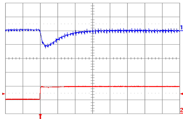
Fig. 1.5V.7: Output voltage response for V_{out} = 1.5V to positive load current step change from 5A to 10A with slew rate of 5A/\mu s at V_{in} = 12V . Top trace: output voltage (100mV/div.); Bottom trace: load current (5A/div.). C_o = 100\mu F ceramic. Time scale: 20\mu s /div.
