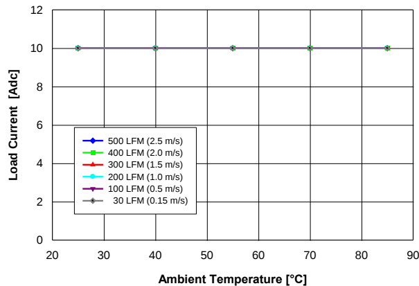
Fig. 1.0V.1: Available load current vs. ambient temperature and airflow rates for V_{out} = 1.0V converter mounted vertically with V_{in} = 12V , and maximum MOSFET temperature \leq 120^\circ C .
