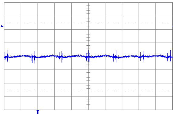
Fig. 1.0V.6: Output voltage ripple (20mV/div.) at full rated load current into a resistive load with external capacitance 100\mu F ceramic and V_{in} = 12V for V_{out} = 1.0V . Time scale: 2μs/div.
