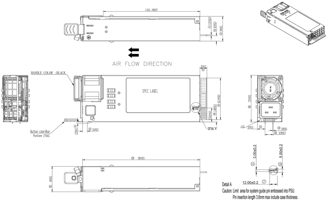
Figure 13. Mechanical Drawing
