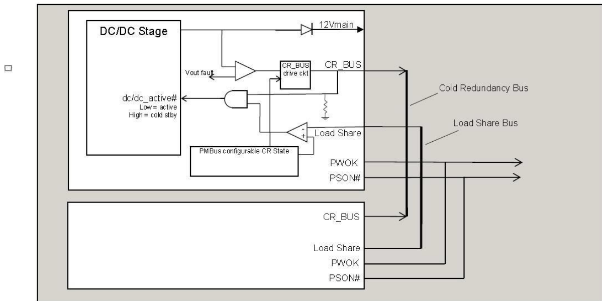
Figure 10. Cold Redundancy 1+1 Functional Block Diagram
