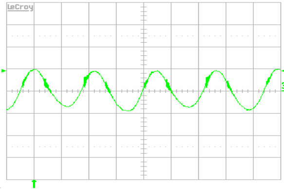
Figure 13. Input reflected ripple-current, i_C (50mA/div.), measured at input terminals at full rated load current and V_{in} = 48V . Refer to Figure 11 for test setup. Time scale: 1μs/div.
