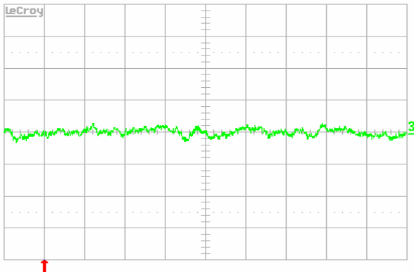
Figure 12. Input reflected-ripple current, i_S (10mA/div.), measured through 10μH at the source at full rated load current and V_{in} = 48V . Refer to Figure 11 for test setup. Time scale: 1μs/div.
