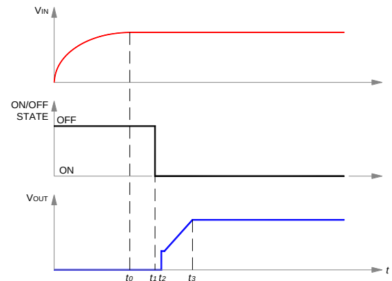
Fig. C: Startup scenario #2
