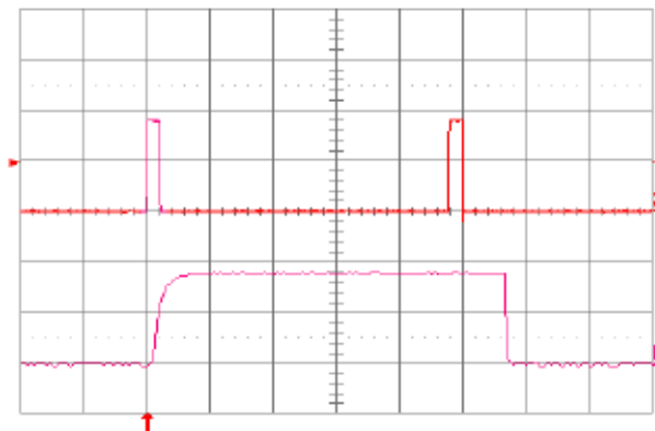
Fig. 1.8V.16: Load current (top trace, 20 A/div., 50 ms/div.) into a 10 m \Omega short circuit during restart, at V_{in} = 48 V. Bottom trace (20 A/div., 2 ms/div.) is an expansion of the on-time portion of the top trace.
