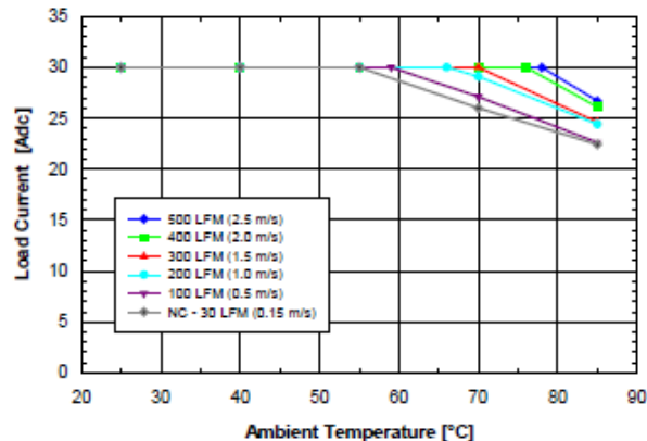
Fig. 1.8V.1: Available load current vs. ambient air temperature and airflow rates for SQE48T30018 converter mounted vertically with air flowing from pin 3 to pin 1, MOSFET temperature \leq 120^\circ\text{C} , V_{in} = 48\text{ V} .
