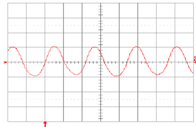
Fig. 3.3V.13: Input reflected-ripple current, i_c (50 mA/div.), measured at input terminals at full rated load current and V_{in} = 48 V. Refer to Fig. 3.3V.12 for test setup. Time scale: 1 \mu s/div.
