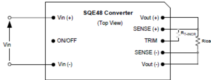
Fig. C: Configuration for increasing output voltage
