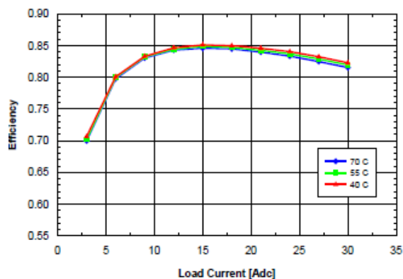
Fig. 1.2V.4: Efficiency vs. load current and ambient temperature for SQE48T30012 converter mounted vertically with Vin = 48 V and air flowing from pin 3 to pin 1 at a rate of 200 LFM (1.0 m/s).
