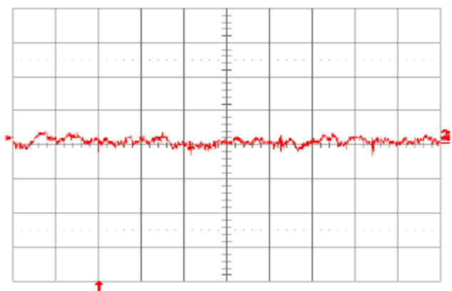
Fig. 1.5V.14: Input reflected-ripple current, i_s (10 mA/div.), measured through 10 \mu H at the source at full rated load current and V_{in} = 48 V. Refer to Fig. 1.5V.12 for test setup. Time scale: 1 \mu s/div
