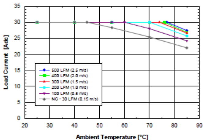
Fig. 1.5V.2: Available load current vs. ambient air temperature and airflow rates for SQE48T30015 converter mounted horizontally with air flowing from pin 3 to pin 1, MOSFET temperature \leq 120 °C, V_{in} = 48 V.
