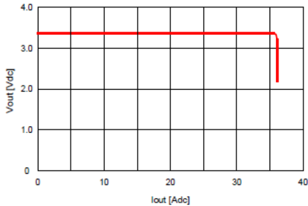
Fig. 3.3V.15: Output voltage vs. load current showing current limit point and converter shutdown point. Input voltage has almost no effect on current limit characteristic.
