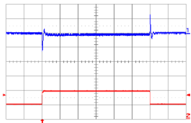
Fig. 1.2V.10: Output voltage response to load current step-change (10 A – 20 A – 10 A) at V_{in} = 48\text{ V} . Top trace: output voltage (100 mV/div.). Bottom trace: load current (10 A/div.). Current slew rate: 0.1 A/ \mu\text{s} . C_o = 1\text{ }\mu\text{F} ceramic. Time scale: 0.2 ms/div.
