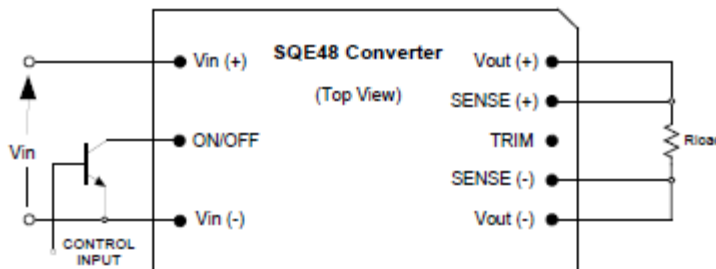
Fig. A: Circuit configuration for ON/OFF function
