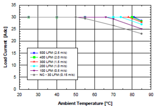
Fig. 1.2V.2: Available load current vs. ambient air temperature and airflow rates for SQE48T30012 converter mounted horizontally with air flowing from pin 3 to pin 1, MOSFET temperature \leq 120 °C, Vin = 48 V.
