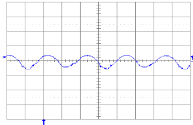
Fig. 1.2V.13: Input reflected ripple-current, i_c (100 mA/div.), measured at input terminals at full rated load current and V_{in} = 48\ \text{V} . Refer to Fig. 1.2V.12 for test setup. Time scale: 1\ \mu\text{s}/\text{div} .
