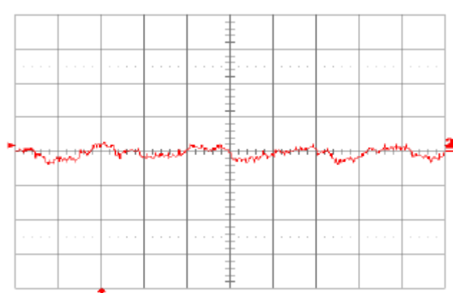
Fig. 3.3V.14: Input reflected-ripple current, i_s (10 mA/div.), measured through 10 \mu H at the source at full rated load current and V_{in} = 48 V. Refer to Fig. 3.3V.12 for test setup. Time scale: 1 \mu s/div
