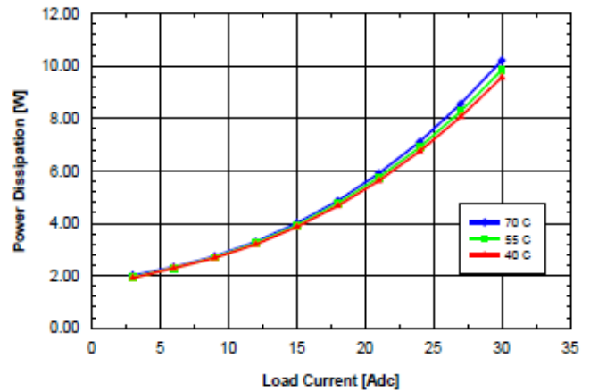
Fig. 2.5V.6: Power dissipation vs. load current and ambient temperature for SQE48T30025 converter mounted vertically with V_{in} = 48\text{ V} and air flowing from pin 3 to pin 1 at a rate of 200 LFM (1.0 m/s).
