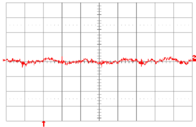
Fig. 1.2V.14: Input reflected-ripple current, i_s (10 mA/div.), measured through 10\ \mu\text{H} at the source at full rated load current and V_{in} = 48\ \text{V} . Refer to Fig. 1.2V.12 for test setup. Time scale: 1\ \mu\text{s}/\text{div} .
