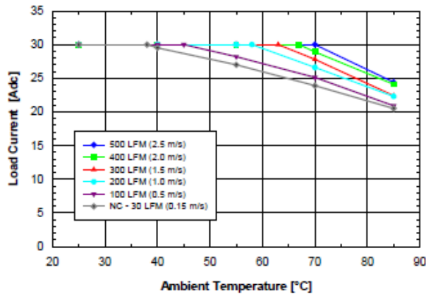
Fig. 2.5V.1: Available load current vs. ambient air temperature and airflow rates for SQE48T30025 converter mounted vertically with air flowing from pin 3 to pin 1, MOSFET temperature ≤ 120 °C, Vin = 48 V.
