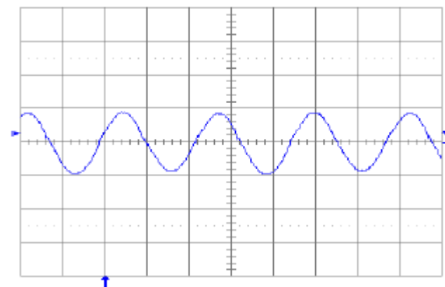
Fig. 3.3V.11: Output voltage ripple (20 mV/div.) at full rated load current into a resistive load with C_o = 10 \mu F tantalum + 1 \mu F ceramic and V_{in} = 48 V. Time scale: 1 \mu s/div..
