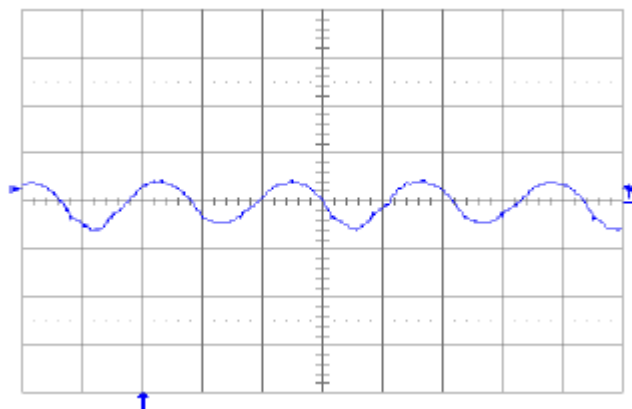
Fig. 1.8V.11: Output voltage ripple (20 mV/div.) at full rated load current into a resistive load with C_o = 10 \mu F tantalum + 1 \mu F ceramic and V_{in} = 48 V. Time scale: 1 \mu s/div.
