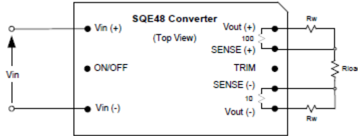
Fig. B: Remote sense circuit configuration
