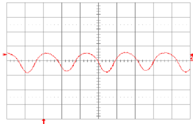
Fig. 1.5V.13: Input reflected ripple-current, i_c (100 mA/div.), measured at input terminals at full rated load current and V_{in} = 48 V. Refer to Fig. 1.5V.12 for test setup. Time scale: 1 \mu s/div.
