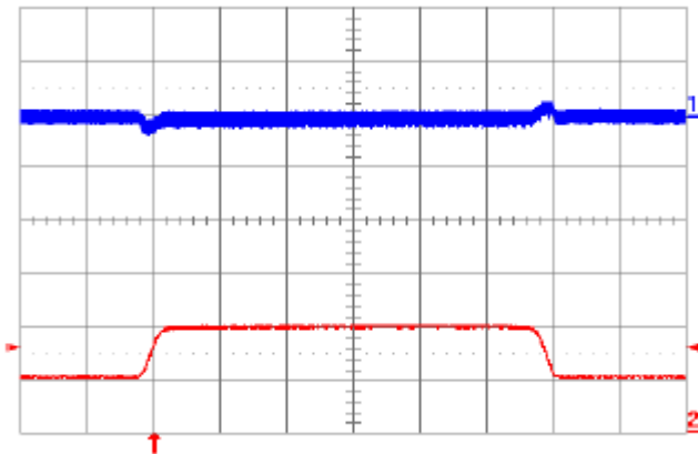
Fig. 1.2V.9: Output voltage response to load current step-change (10 A – 20 A – 10 A) at V_{in} = 48\text{ V} . Top trace: output voltage (100 mV/div.). Bottom trace: load current (10 A/div.). Current slew rate: 0.1 A/ \mu\text{s} . C_o = 1\text{ }\mu\text{F} ceramic. Time scale: 0.2 ms/div.
