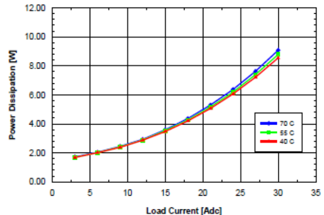
Fig. 1.8V.6: Power dissipation vs. load current and ambient temperature for SQE48T30018 converter mounted vertically with V_{in} = 48\text{ V} and air flowing from pin 3 to pin 1 at a rate of 200 LFM (1.0 m/s).
