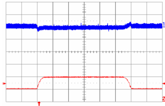
Fig. 3.3V.9: Output voltage response to load current step-change (10 A – 20 A – 10 A) at V_{in} = 48 V. Top trace: output voltage (100 mV/div.). Bottom trace: load current (10 A/div.). Current slew rate: 0.1 A/ \mu s. C_o = 1 \mu F ceramic. Time scale: 0.2 ms/div.
