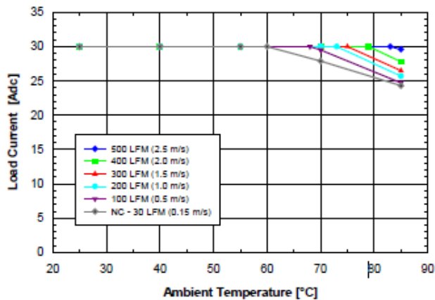
Fig. 1.2V.1: Available load current vs. ambient air temperature and airflow rates for SQE48T30012 converter mounted vertically with air flowing from pin 3 to pin 1, MOSFET temperature \leq 120 °C, Vin = 48 V.
