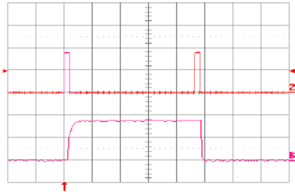
Fig. 1.5V.16: Load current (top trace, 20 A/div., 50 ms/div.) into a 10 mΩ short circuit during restart, at Vin = 48 V. Bottom trace (20 A/div., 2 ms/div.) is an expansion of the on-time portion of the top trace.
