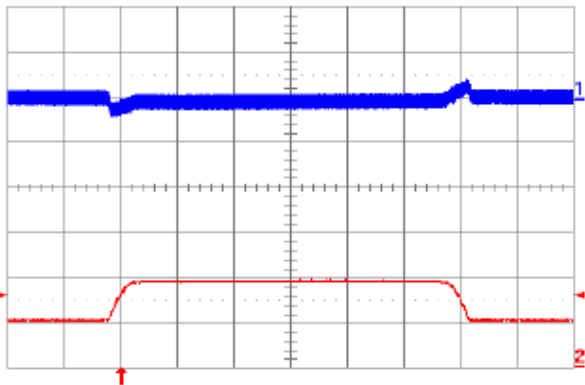
Fig. 2.5V.9: Output voltage response to load current step-change (10 A – 20 A – 10 A) at V_{in} = 48\text{ V} . Top trace: output voltage (100 mV/div.). Bottom trace: load current (10 A/div.). Current slew rate: 0.1\text{ A}/\mu\text{s} . C_o = 1\text{ }\mu\text{F} ceramic. Time scale: 0.2 ms/div.
