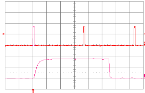
Fig. 3.3V.16: Load current (top trace, 20 A/div., 50 ms/div.) into a 10 mΩ short circuit during restart, at Vin = 48 V. Bottom trace (20 A/div., 1 ms/div.) is an expansion of the on-time portion of the top trace.
