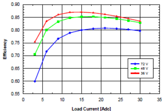
Fig. 1.2V.3: Efficiency vs. load current and input voltage for SQE48T30012 converter mounted vertically with air flowing from pin 3 to pin 1 at a rate of 300 LFM (1.5 m/s) and Ta = 25 °C.
