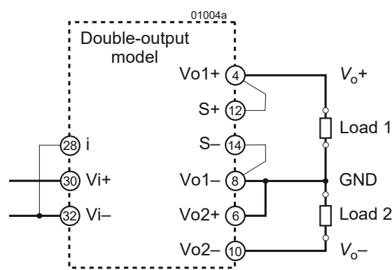
Fig. 4 Symmetrical-output configuration (with common ground)
