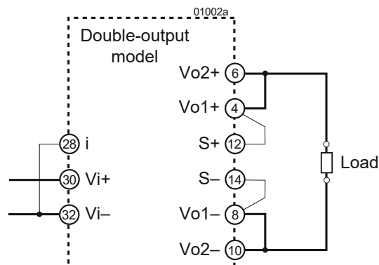
Fig. 2 Parallel-output configuration
