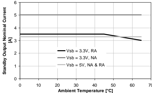
Figure 23. Temperature derating on V_{SB}
