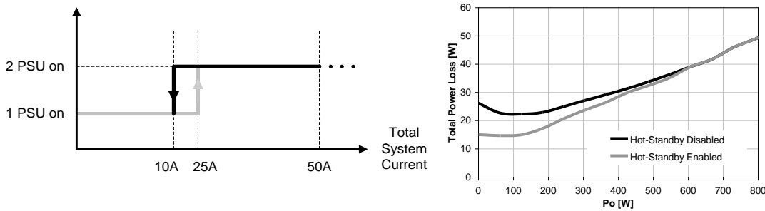
Figure 30. Hot-standby enable/disable current thresholds
