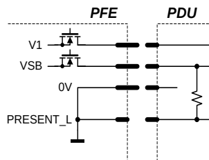
Figure 11. PRESENT_L signal pin
