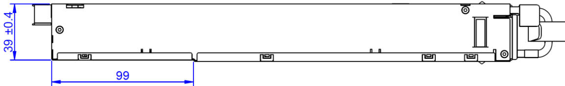
Figure 28. Side View 2
