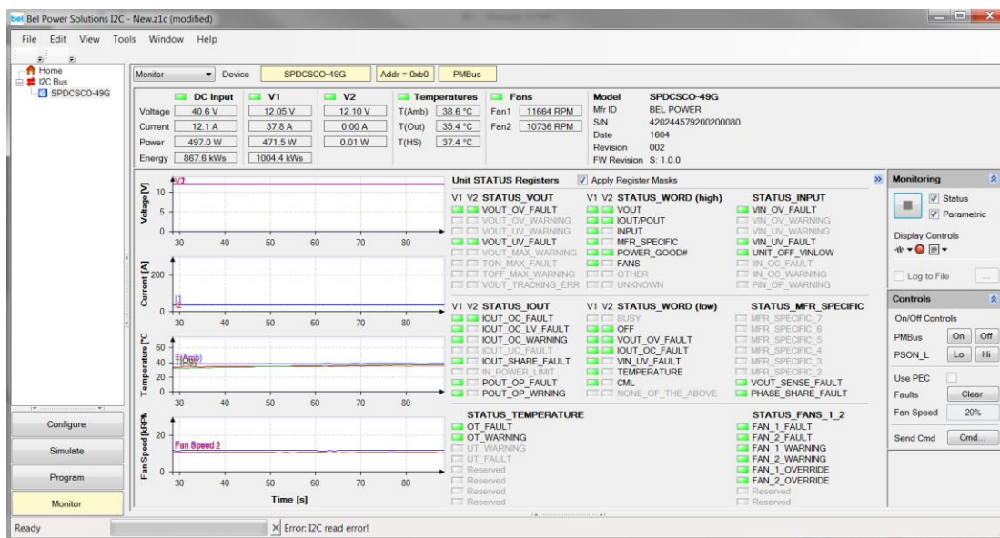
Figure 17. Monitoring dialog of the I 2 C Utility
