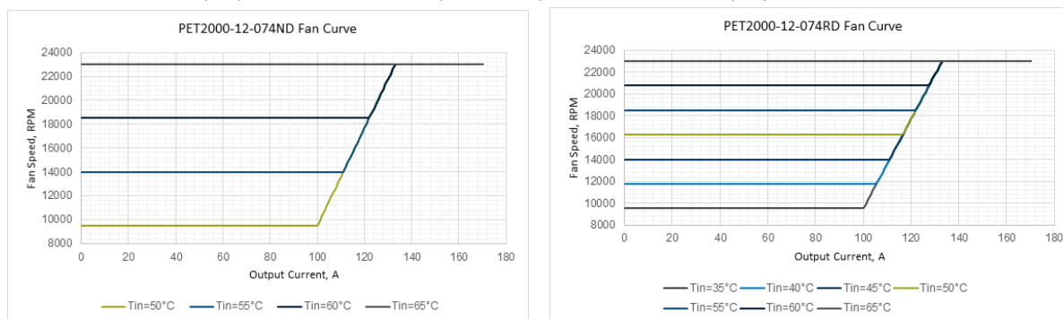
Figure 20. Fan speed vs. main output load
