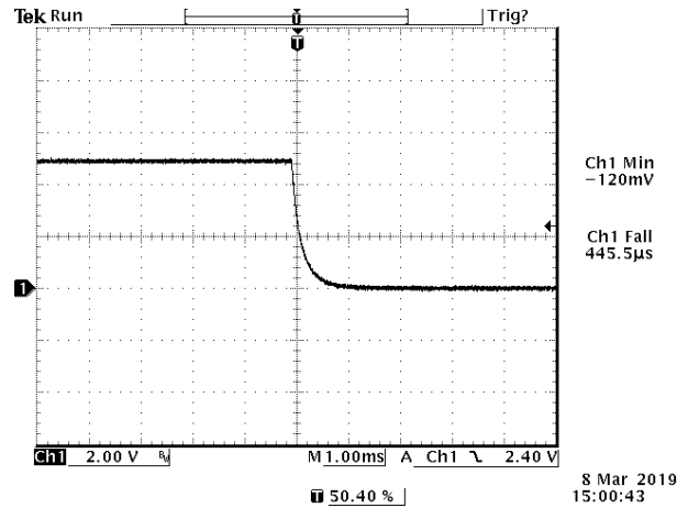
Figure 35. Typical Shut down From Venable
