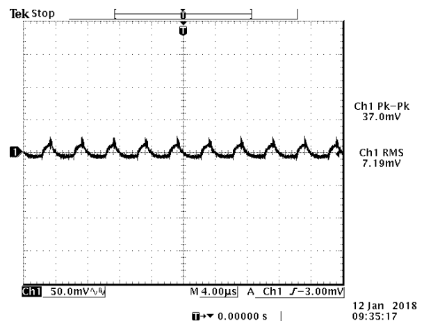
Figure 17. Ripple and noise at V_{in} = 110 V 5 Vdc/10 A output @ T_a = 25^\circ\text{C} with C_{ext} = 200 \mu F
