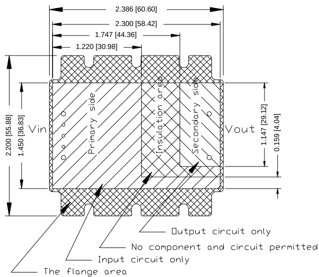
Figure 58. 0RQB-50Y05E/F Recommended pad layout-1
