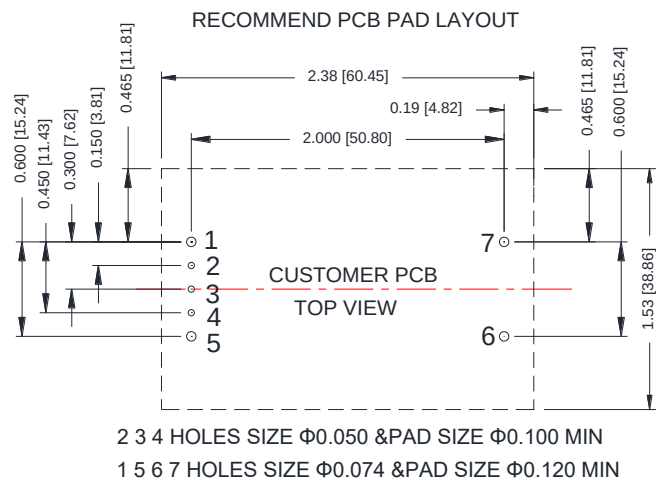
Figure 55. 0RQB-50Y05L/0 Recommended pad layout-2
