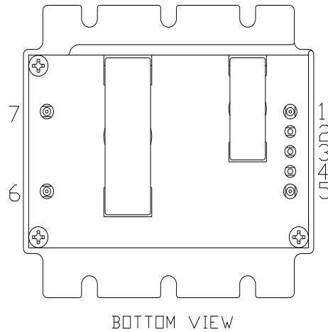
Figure 57. 0RQB-50Y05E/F Pins
