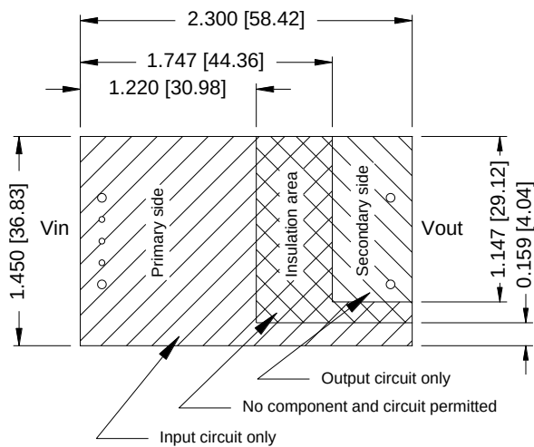
Figure 54. 0RQB-50Y05L/0 Recommended pad layout-1
