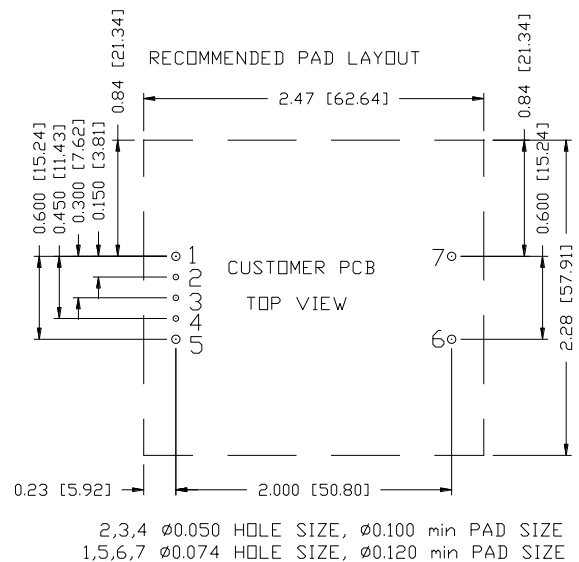
Figure 59. 0RQB-50Y05E/F Recommended pad layout-2
