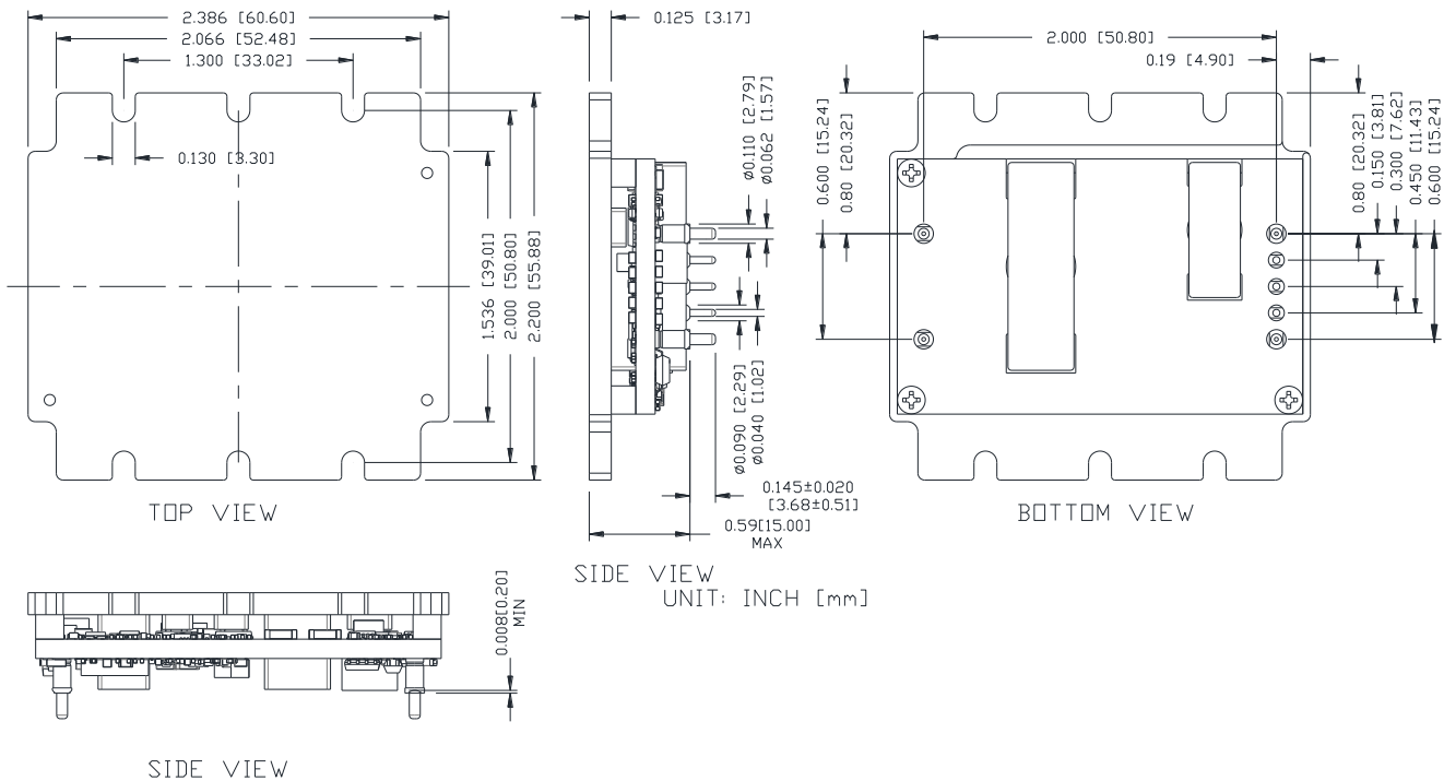
Figure 56. 0RQB-50Y05E/F Outline
