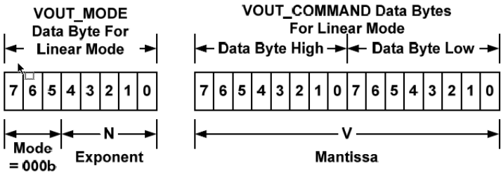
Figure 14. Linear Format Data Bytes
