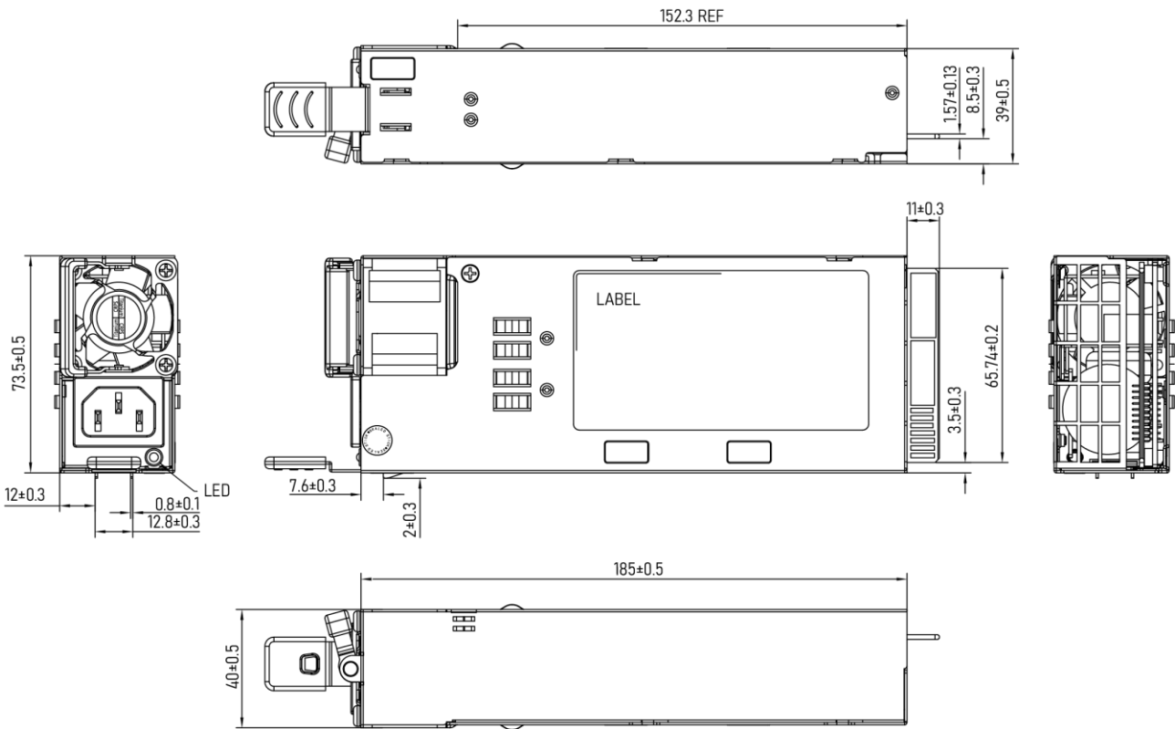
Figure 19. Mechanical Drawing
