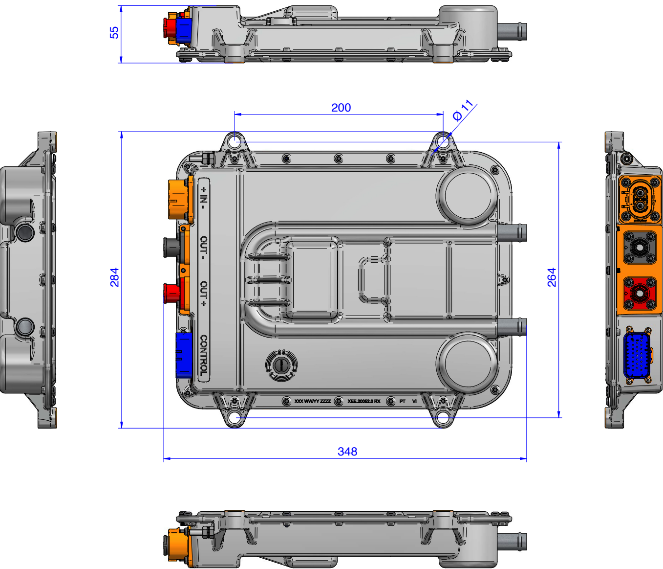
Figure 7. Mechanical Drawing
