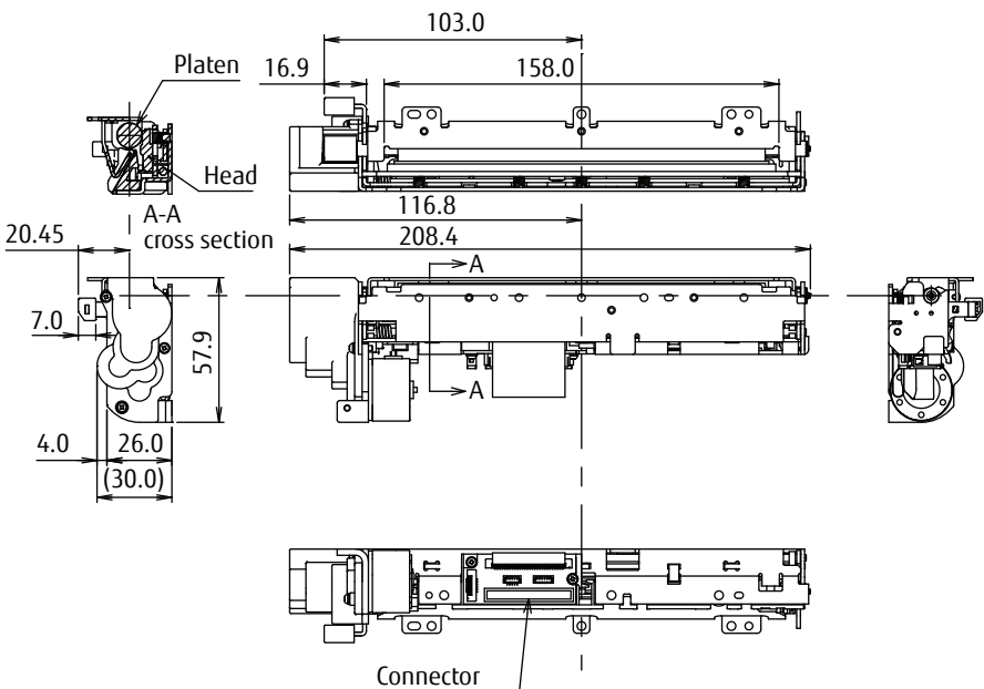
FTP-66EMCL162-R - Low Speed
