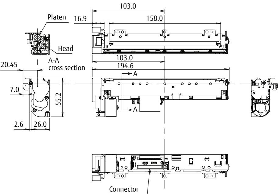
FTP-66EMCL112-R - High Speed
