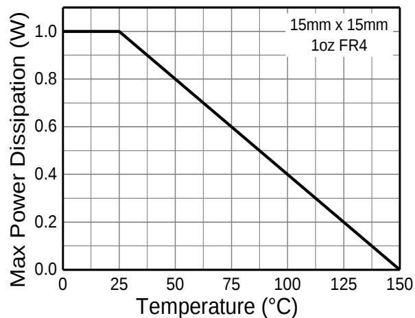
Derating Curve
