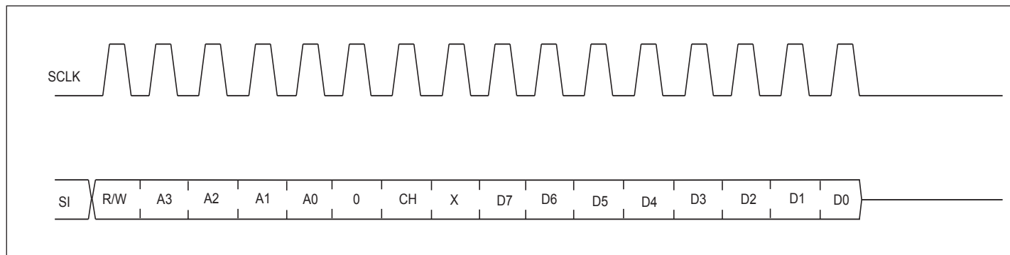
Figure 13. SPI Write
