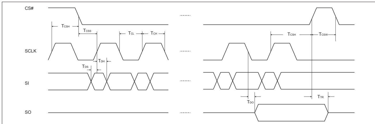
Figure 26. SPI-Bus Timing
