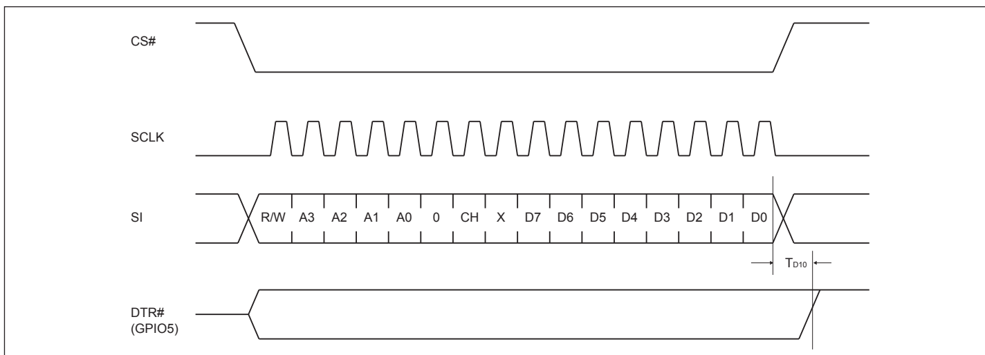
Figure 28. SPI Write MCR to DTR Output Switch
