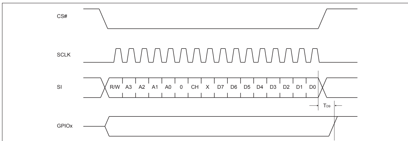
Figure 27. SPI Write MCR to DTR Output Switch
