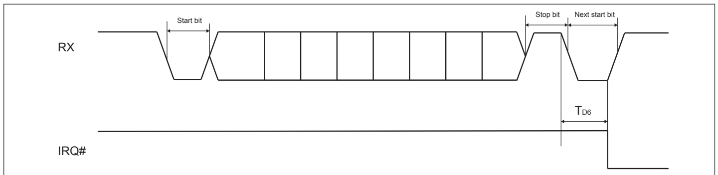
Figure 23. Receive Interrupt
