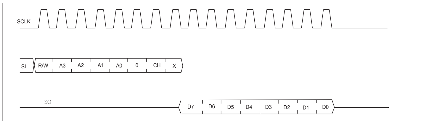
Figure 14. SPI Read
