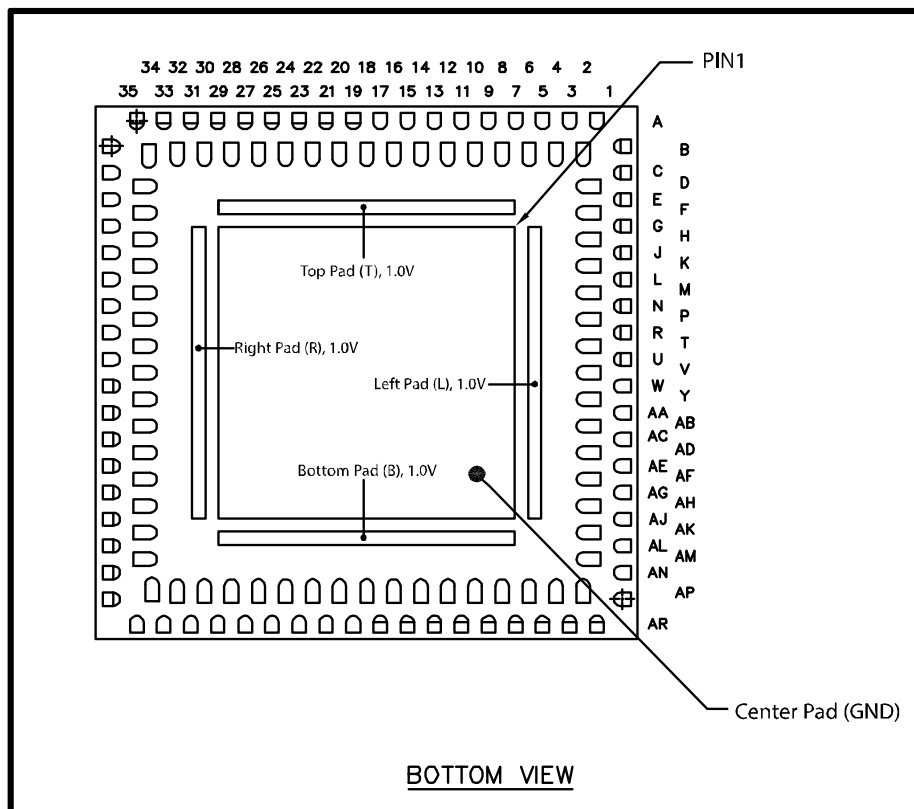
Figure 14-2 Package Bottom View
