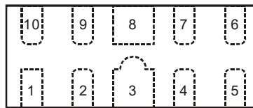
Site 3: U-DFN2510-10 (Type CJ)
