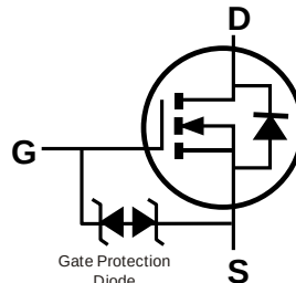
Internal Schematic
