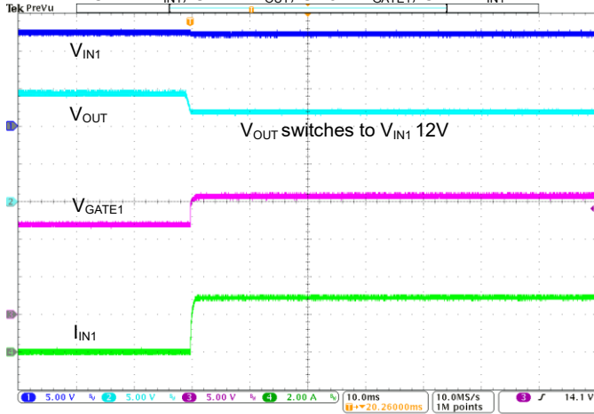
ORing VIN2 to VIN1 Switch Over
