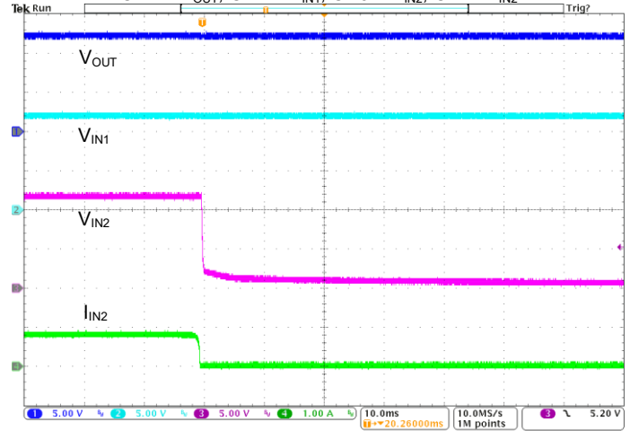
ORing VIN2 Failure and Switch Over to VIN1
