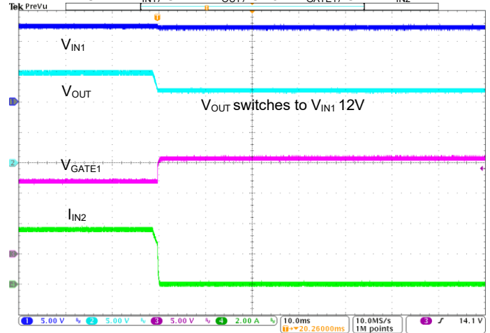
ORing VIN2 to VIN1 Switch Over
