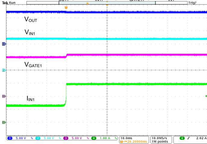
ORing VIN2 Failure and Switch Over to VIN1
