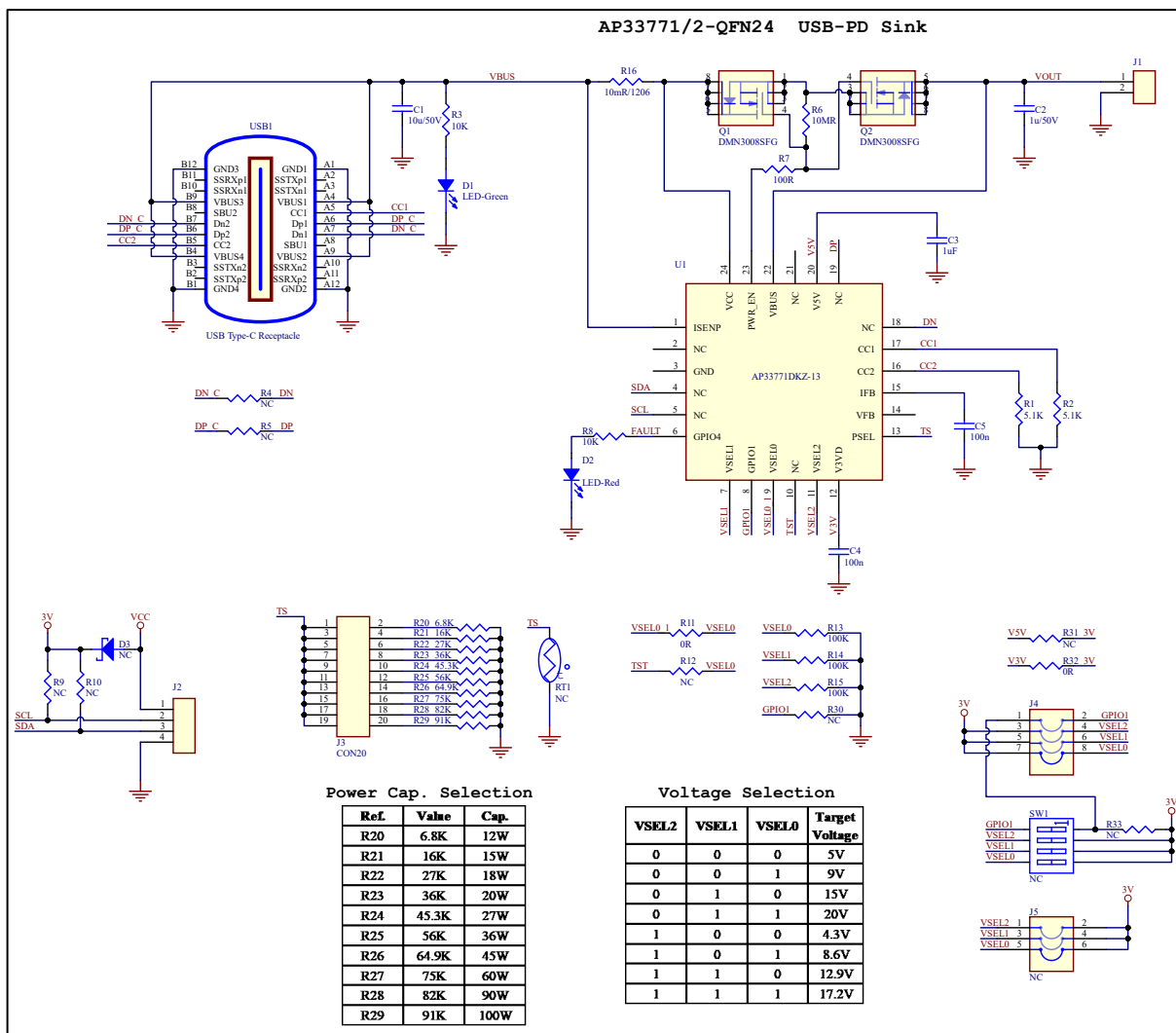
Figure 5: Schematics of the AP33771 Evaluation Board with tables of PDO selection and power capability
