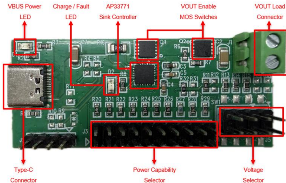
Figure 3: AP33771 evaluation board top view and its key portions
