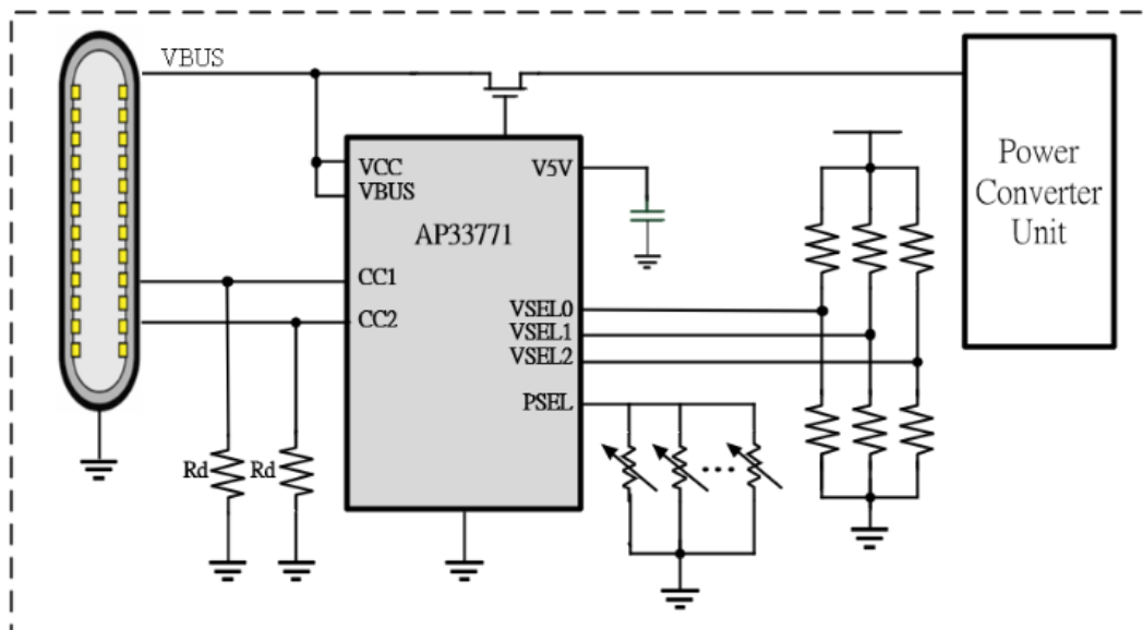
Figure 4: Block diagram of the AP33771 evaluation board
