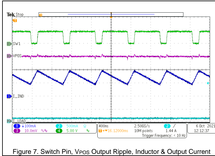
Figure 7. Switch Pin, V_{POS} Output Ripple, Inductor & Output Current
