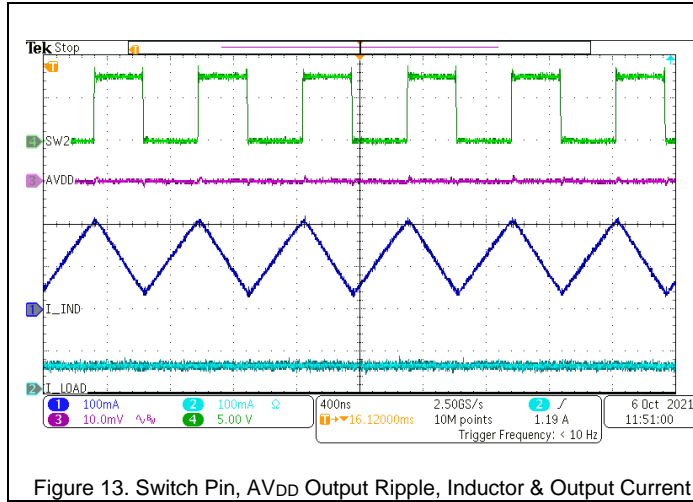
Figure 13. Switch Pin, AV_{DD} Output Ripple, Inductor & Output Current
