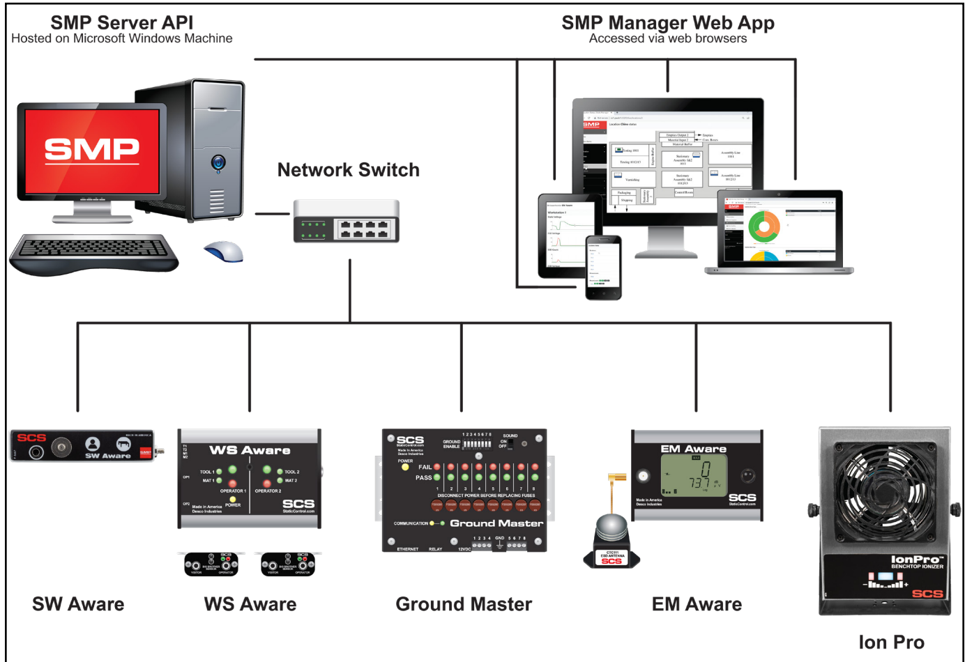
Figure 8. SMP system setup
