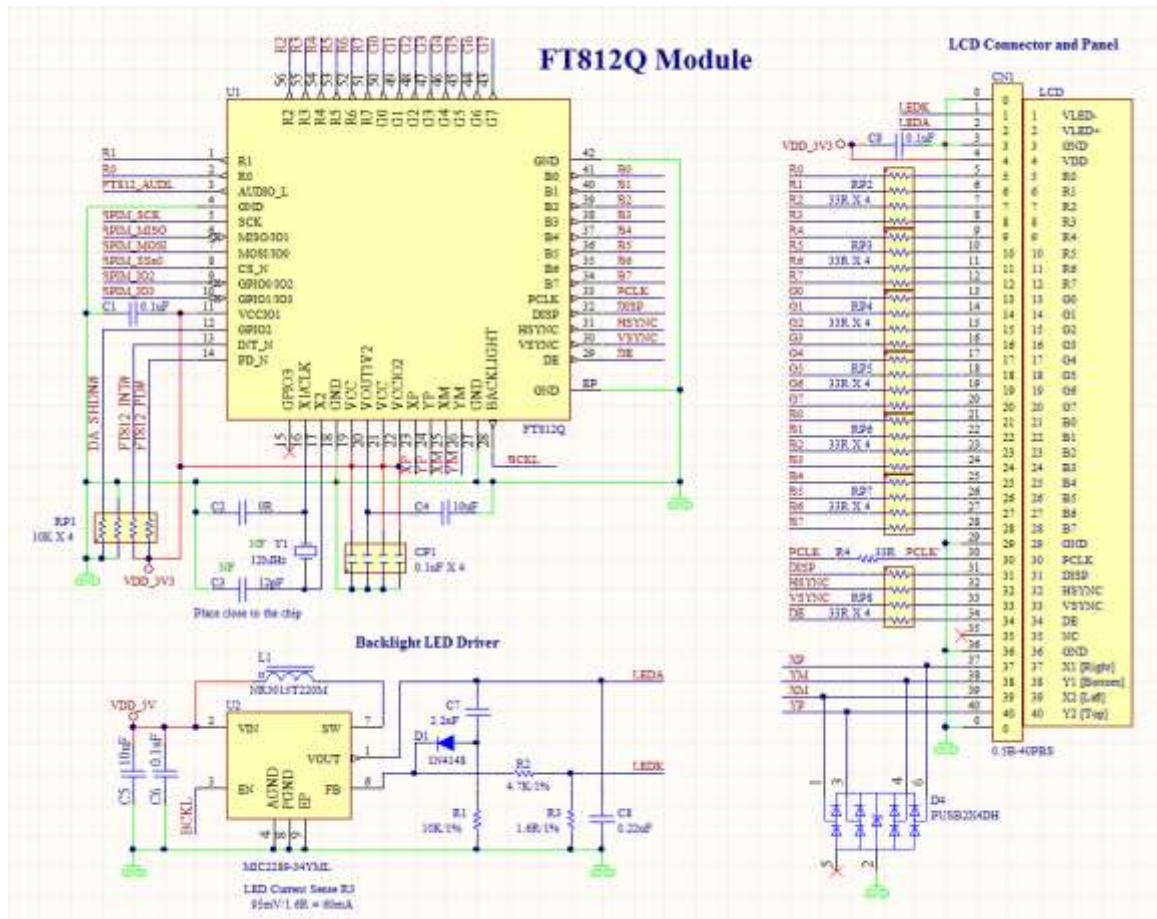
Figure 4 – LCD Interface
