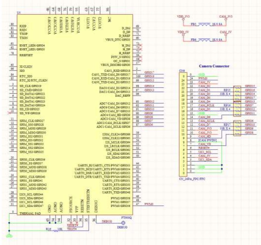
Figure 5 – Camera Interface
