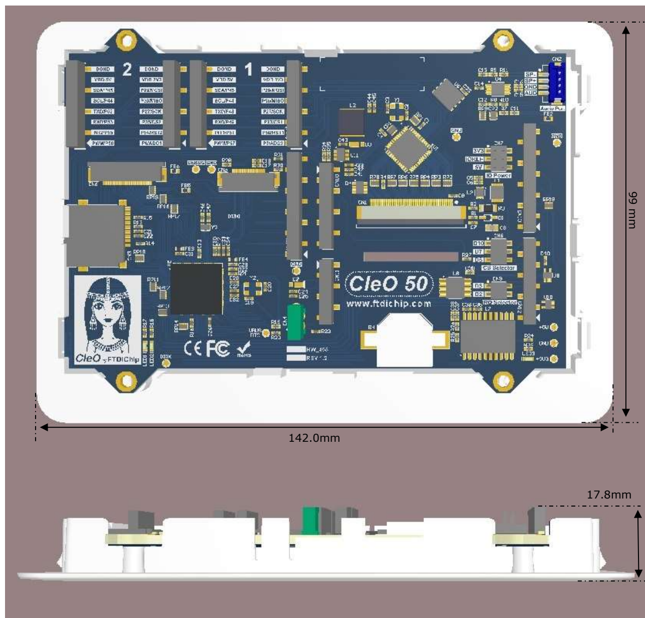
Figure 12 – CleO50 Module Dimensions
