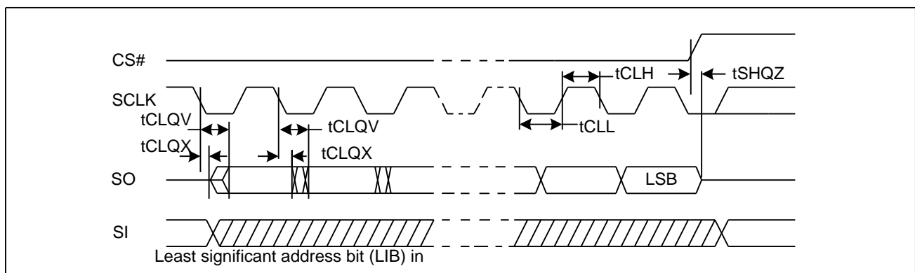
Figure 71. Output Timing
