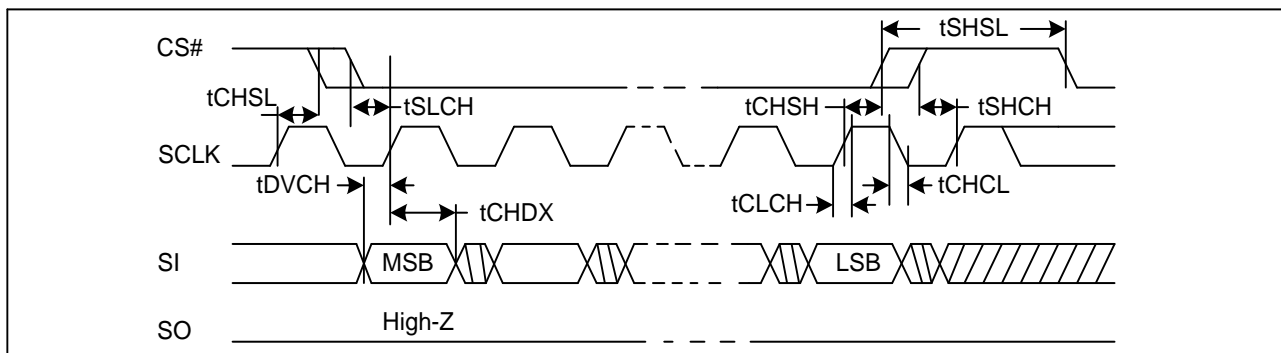
Figure 70. Input Timing
