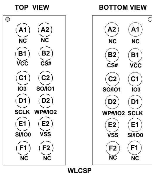
Figure 1 Connection Diagram for WLCSP package
