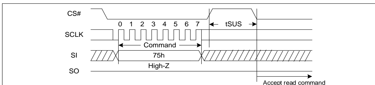
Figure 53. Program/Erase Suspend Sequence Diagram (SPI)
