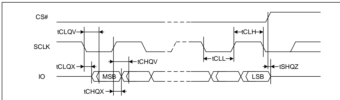
Figure 73. Serial Output Timing (DTR)
