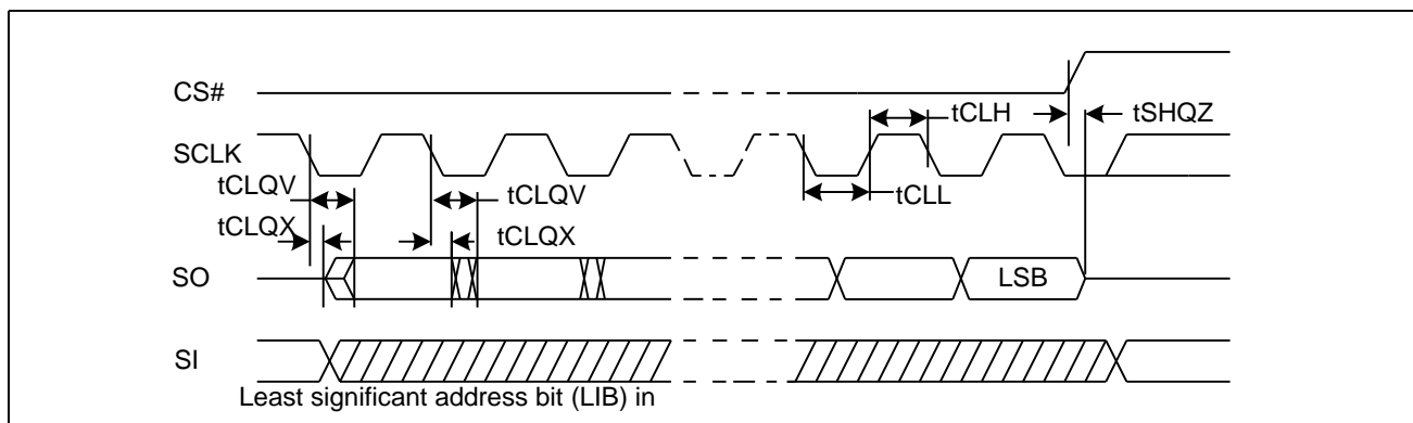
Figure 74. Output Timing
