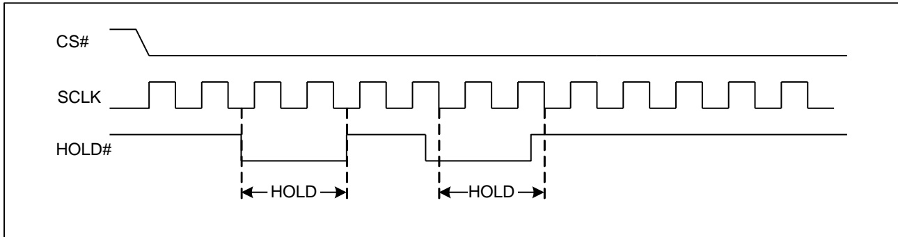
Figure 5 HOLD Condition
