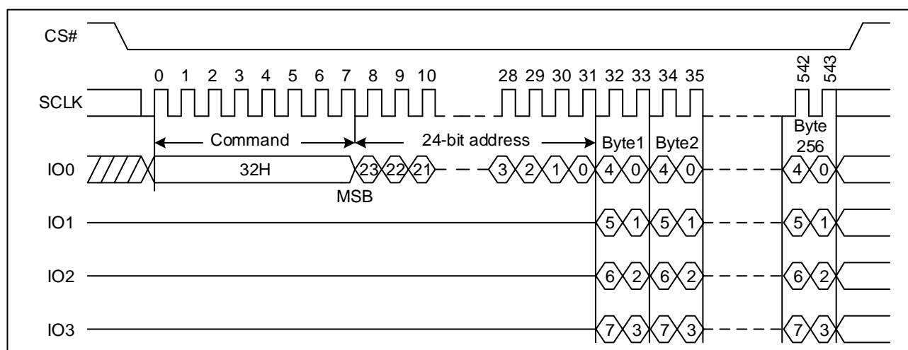
Figure 37. Quad Page Program Sequence Diagram
