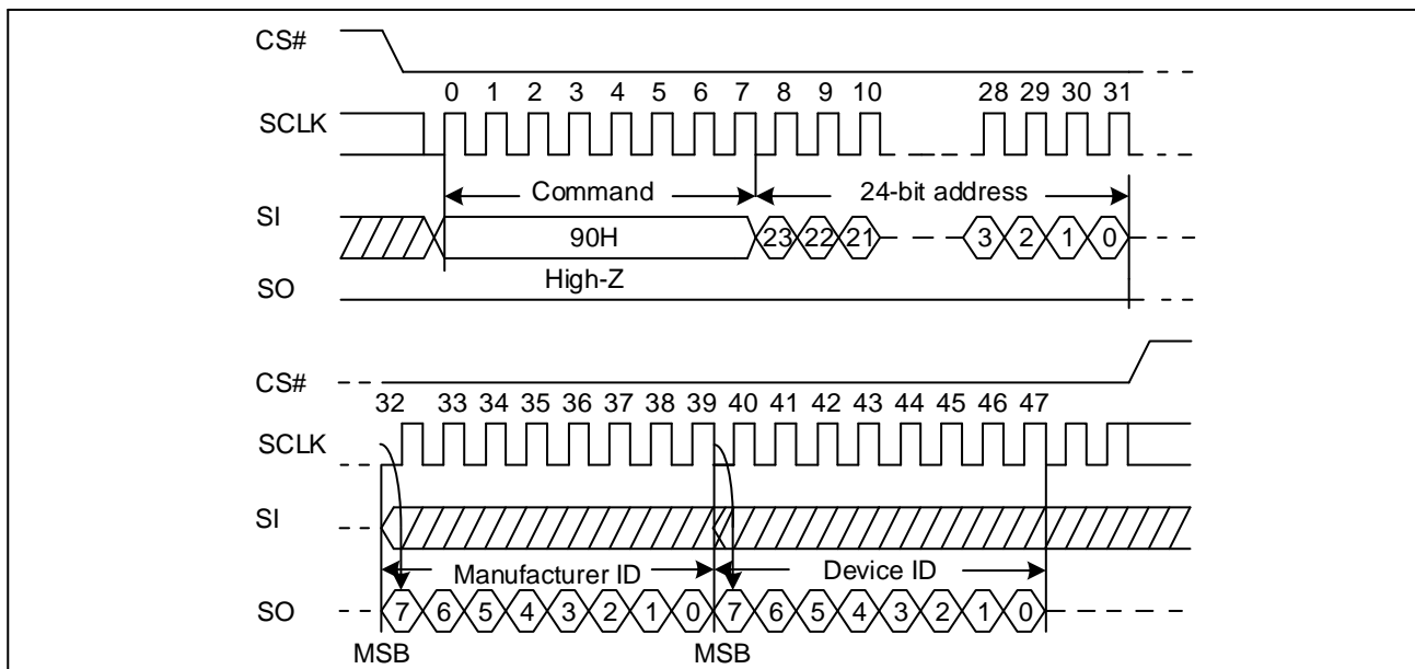
Figure 46. Read Manufacture ID/ Device ID Sequence Diagram (SPI)
