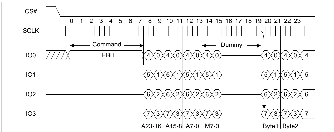
Figure 26. Quad I/O Fast Read Sequence Diagram (SPI, M5-4 ≠ (1, 0))
