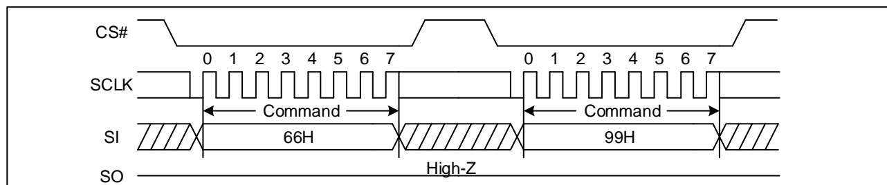
Figure 54. Enable Reset and Reset command Sequence Diagram (SPI)
