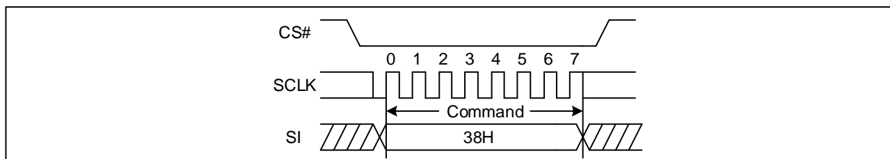
Figure 66. Enable QPI mode command Sequence Diagram
