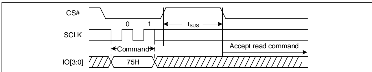
Figure 57. Program/Erase Suspend Sequence Diagram (QPI)
