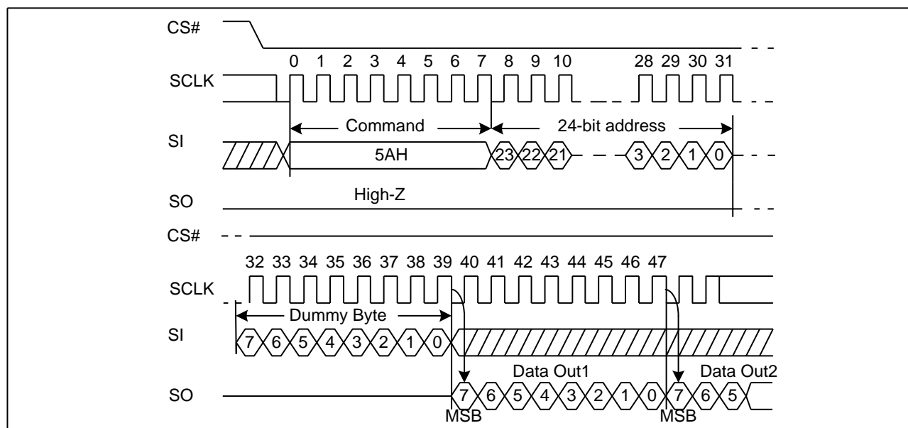
Figure 68. Read Serial Flash Discoverable Parameter command Sequence Diagram
