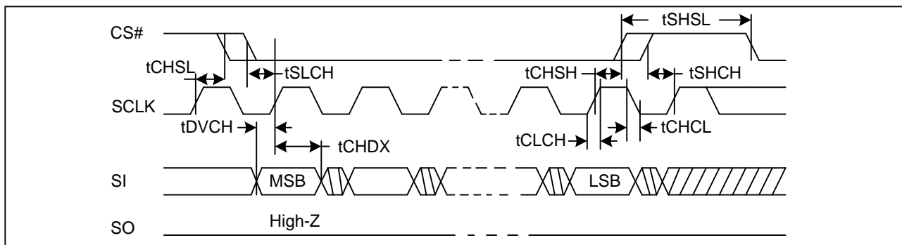
Figure 73. Input Timing
