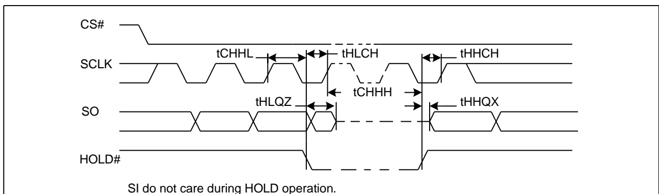
Figure 78. Hold Timing
