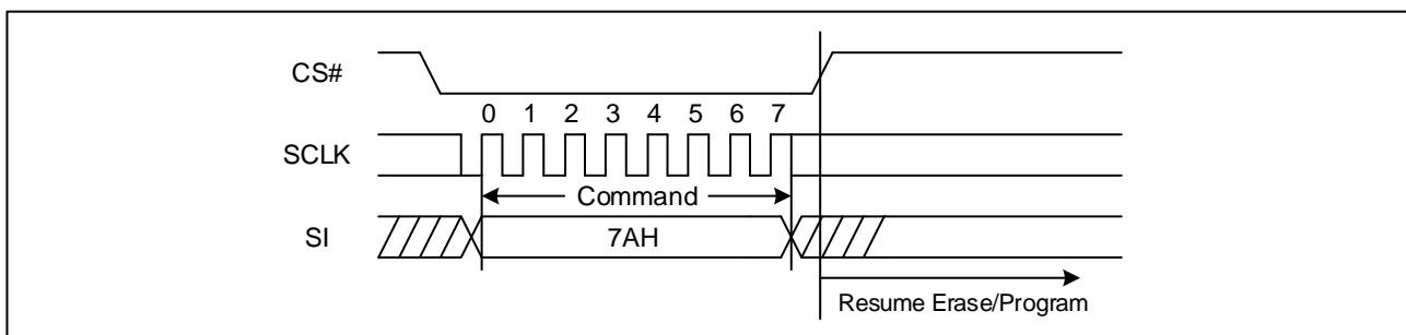
Figure 58. Program/Erase Resume Sequence Diagram (SPI)
