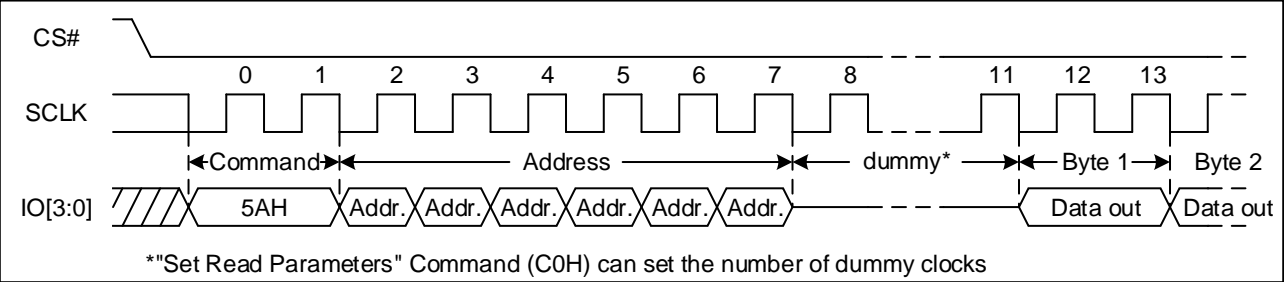
Figure 69. Read Serial Flash Discoverable Parameter command Sequence Diagram (QPI)
