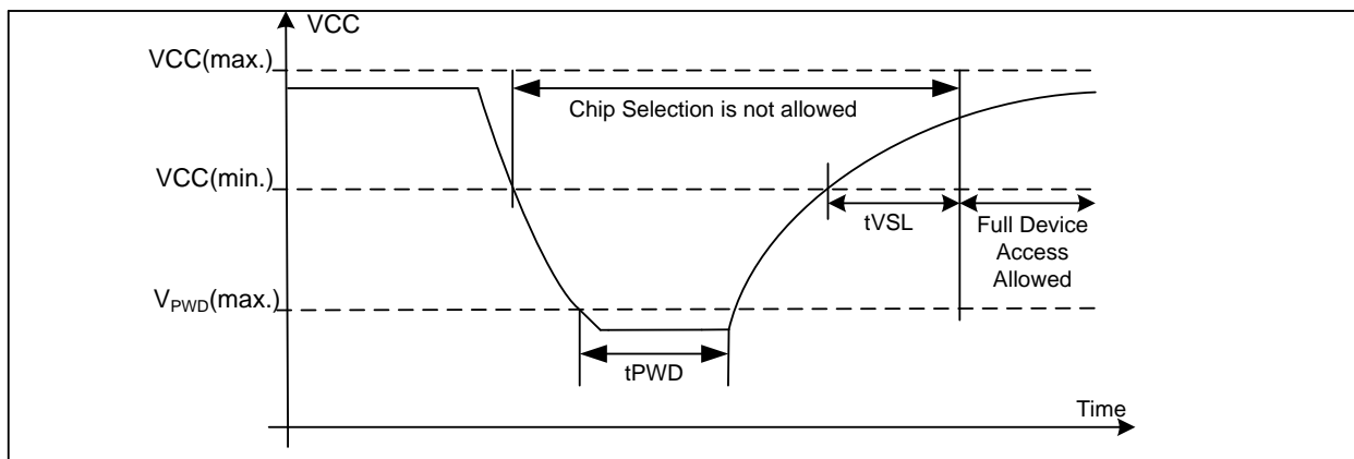
Figure 70. Power-On Timing Sequence Diagram
