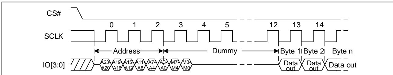
Figure 31. DTR Quad I/O Fast Read Sequence Diagram ((M5-4) = (1, 0))
