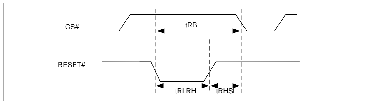
Figure 80 RESET Timing
