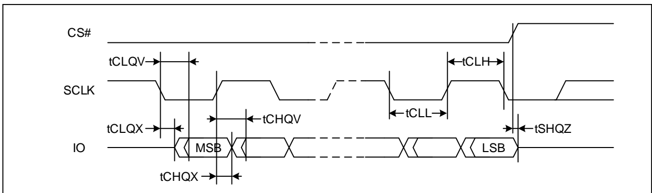
Figure 76. Serial Output Timing (DTR)
