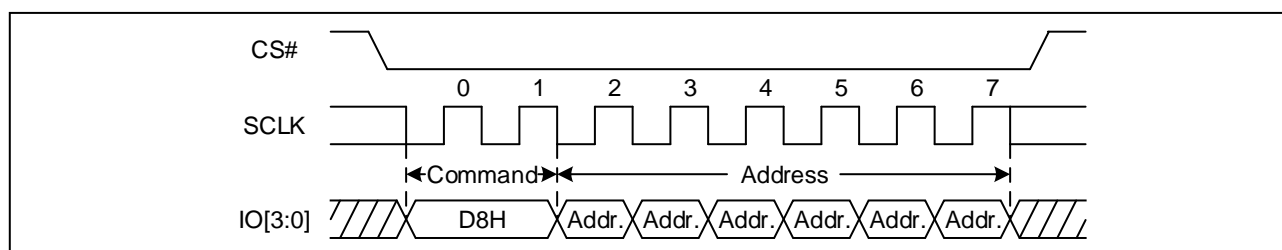
Figure 43. 64KB Block Erase Sequence Diagram (QPI)
