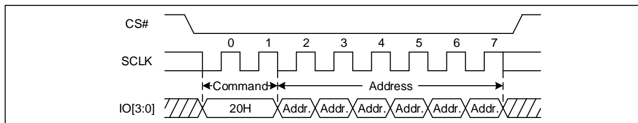
Figure 39. Sector Erase Sequence Diagram (QPI)
