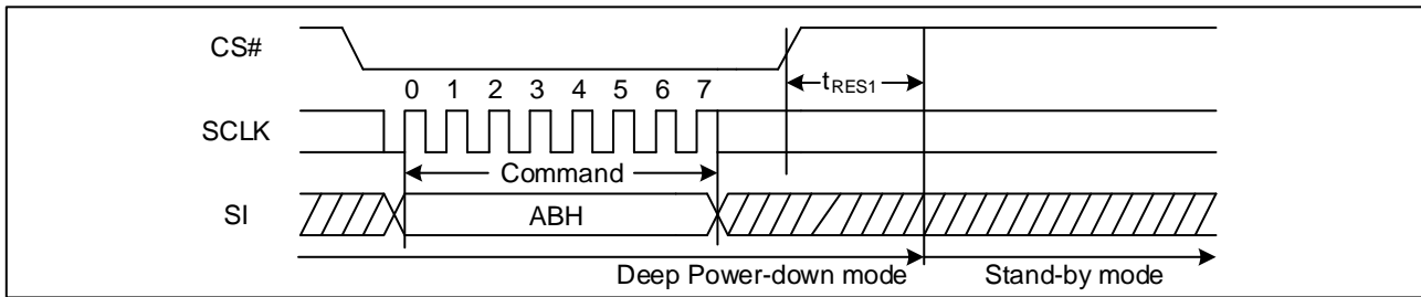
Figure 62. Release Power-Down Sequence Diagram (SPI)
