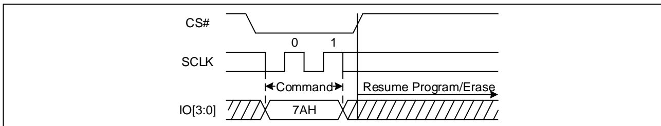
Figure 59. Program/Erase Resume Sequence Diagram (QPI)
