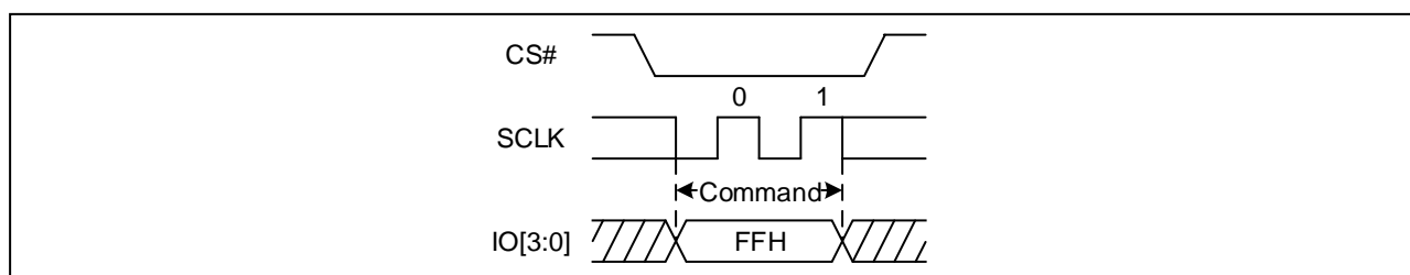
Figure 67. Disable QPI mode command Sequence Diagram
