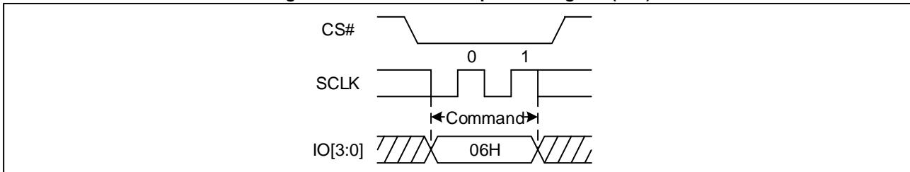
Figure 8. Write Enable Sequence Diagram (QPI)
