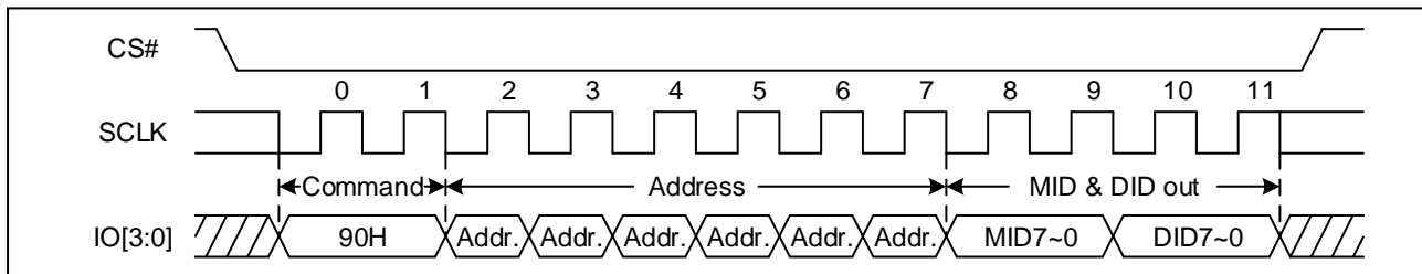
Figure 47. Read Manufacture ID/ Device ID Sequence Diagram (QPI)
