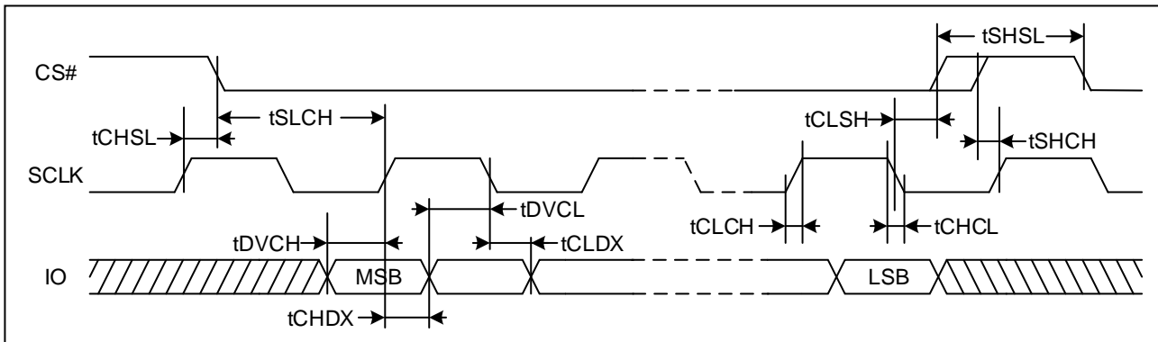
Figure 75. Serial Input Timing (DTR)
