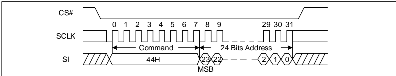
Figure 51. Erase Security Registers command Sequence Diagram
