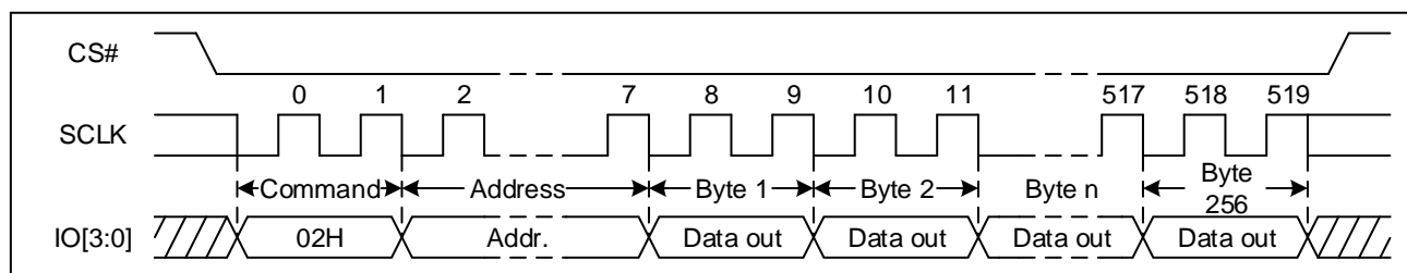
Figure 36. Page Program Sequence Diagram (QPI)
