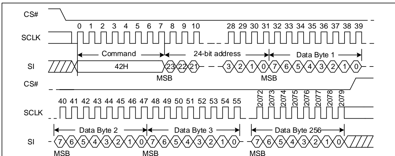
Figure 52. Program Security Registers command Sequence Diagram
