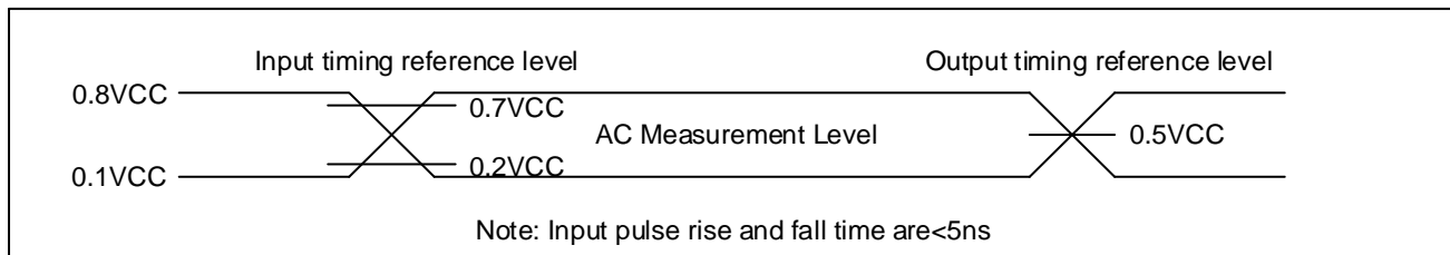
Figure 72. Absolute Maximum Ratings Diagram
