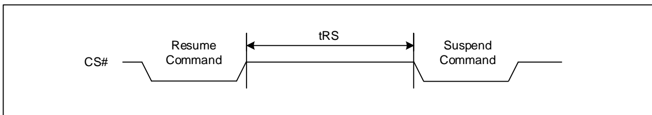
Figure 77. Resume to Suspend Timing Diagram
