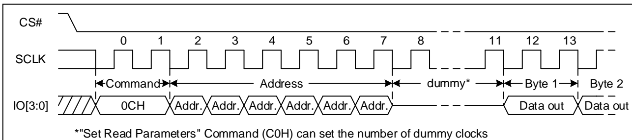
Figure 32. Burst Read with Wrap command Sequence Diagram
