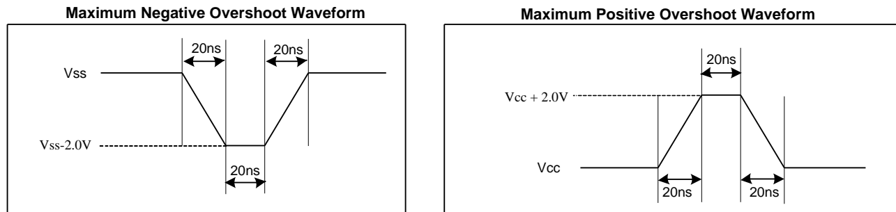
Figure 71. Input Test Waveform and Measurement Level
