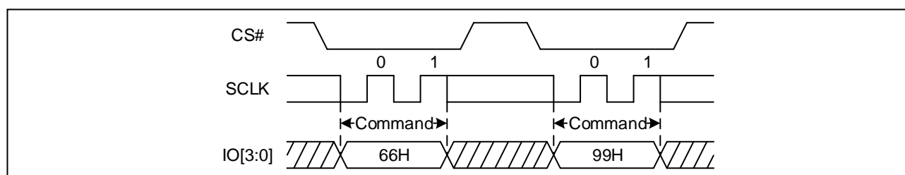
Figure 55. Enable Reset and Reset command Sequence Diagram (QPI)
