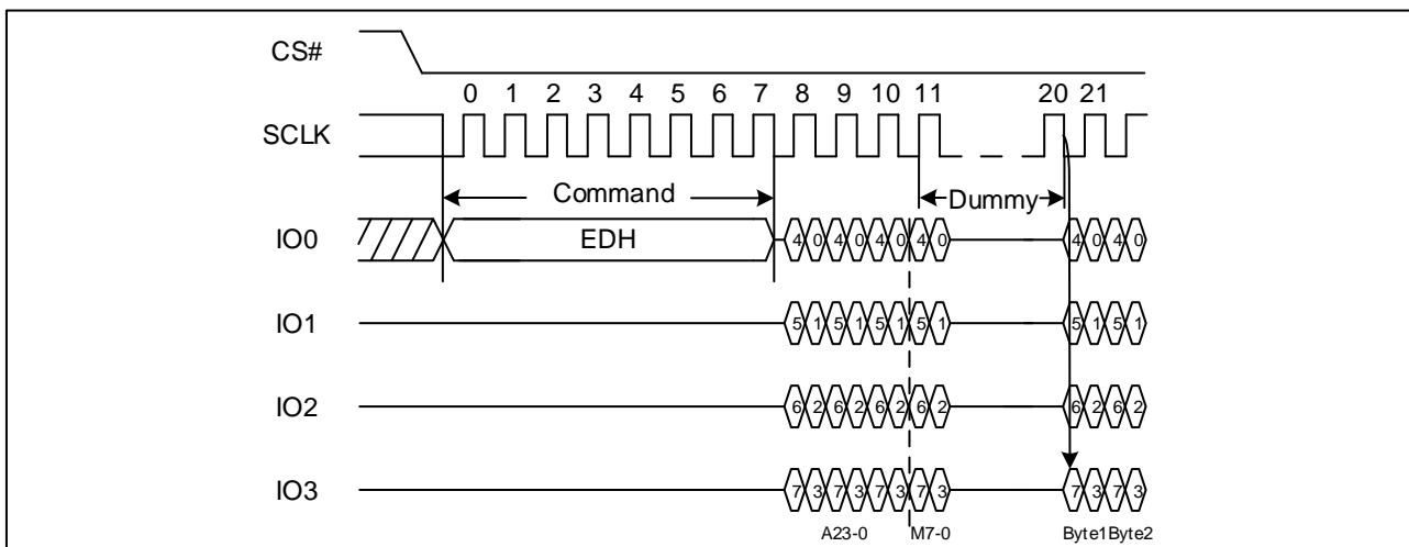
Figure 29. DTR Quad I/O Fast Read Sequence Diagram (SPI, (M5-4) ≠ (1, 0))
