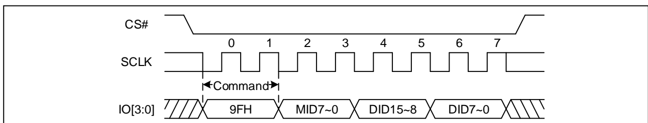
Figure 49. Read Identification ID Sequence Diagram (QPI)
