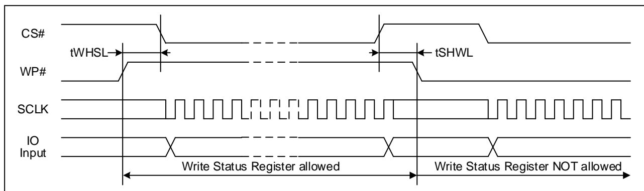
Figure 79. WP# Timing
