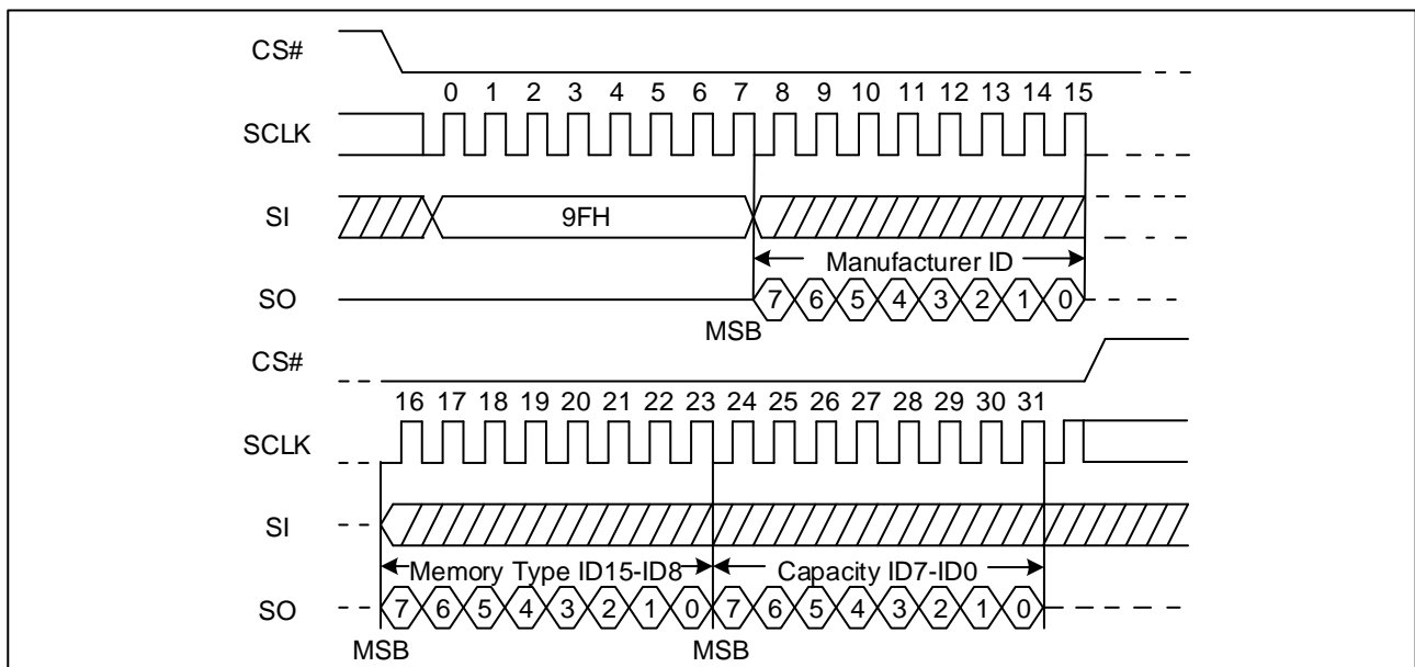
Figure 48. Read Identification ID Sequence Diagram (SPI)
