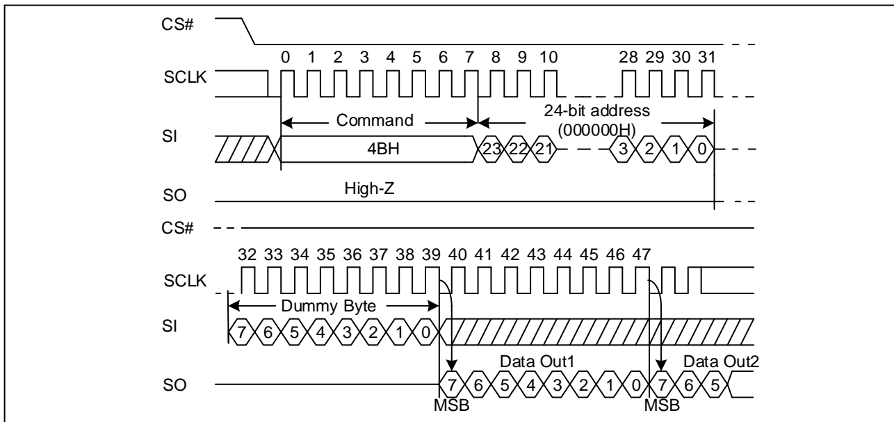
Figure 50. Read Unique ID Sequence Diagram
