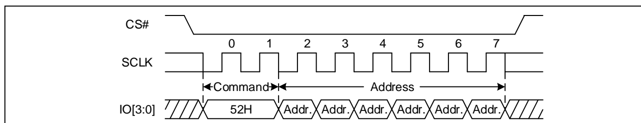
Figure 41. 32KB Block Erase Sequence Diagram (QPI)
