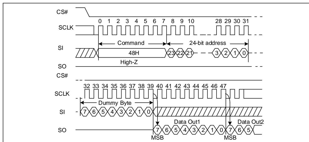
Figure 53. Read Security Registers command Sequence Diagram
