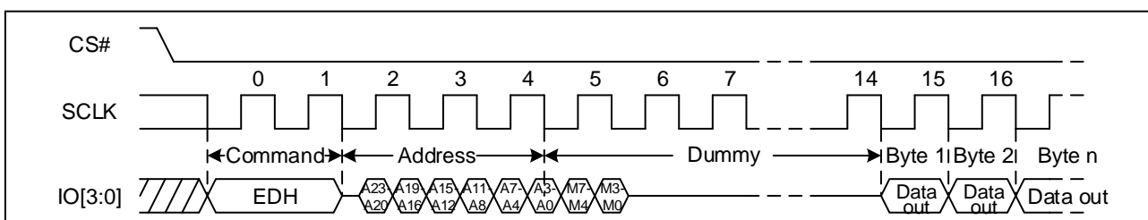
Figure 30. DTR Quad I/O Fast Read Sequence Diagram (QPI, (M5-4) ≠ (1, 0))
