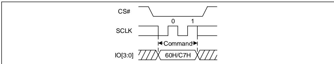
Figure 45. Chip Erase Sequence Diagram (QPI)
