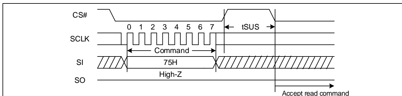
Figure 56. Program/Erase Suspend Sequence Diagram (SPI)
