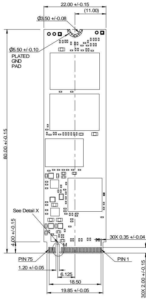
TOP VIEW
