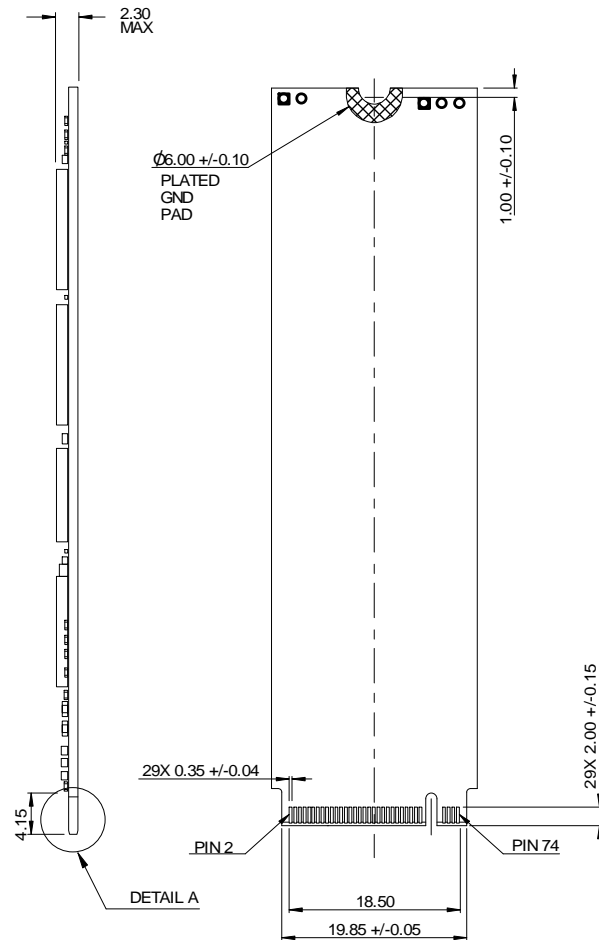
BOTTOM VIEW
