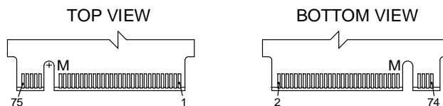
Pin Layout
