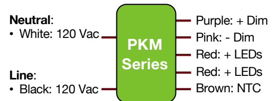
Wiring Diagram
