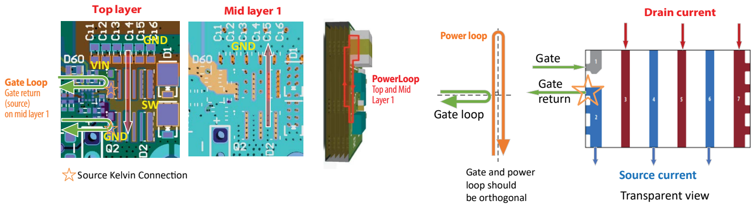
Figure 13: Inner Vertical Layout for Power and Gate Loops from EPC90156
