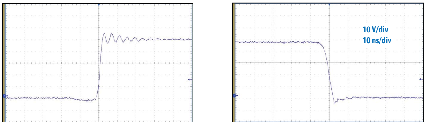
Figure 14: Typical half-bridge voltage switching waveforms
