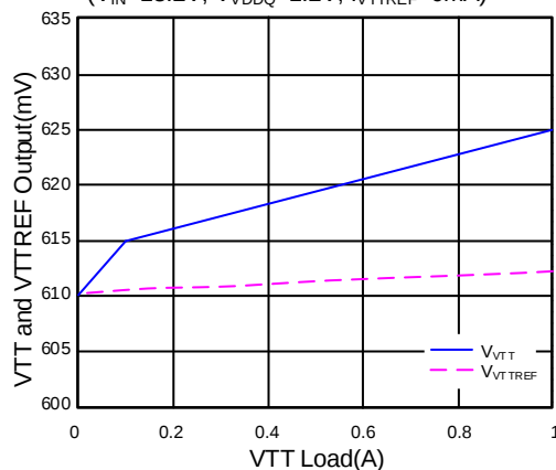
VTT Load Regulation (Sink Current) ( V_{IN}=13.2V , V_{VDDQ}=1.2V , I_{VTTREF}=0mA )
