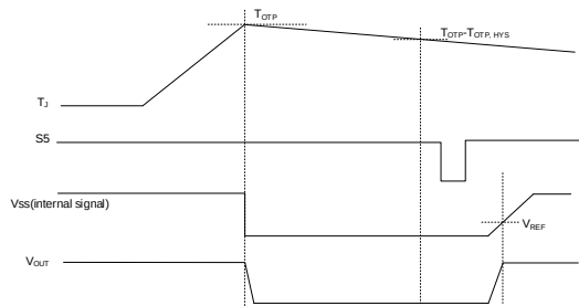
Figure 11. Overtemperature protection
