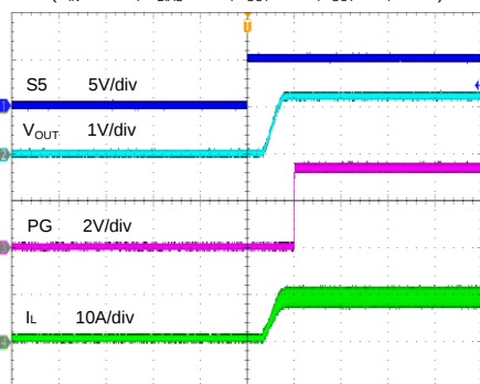
PG Test When S5 On
