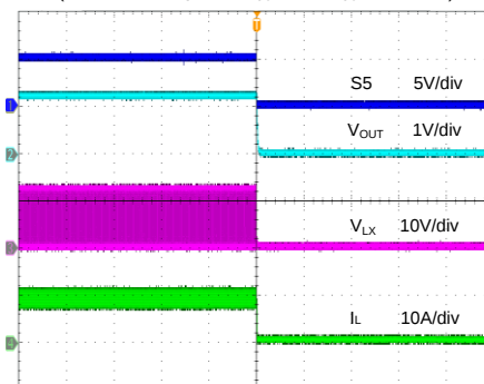
Buck Shutdown from S5
