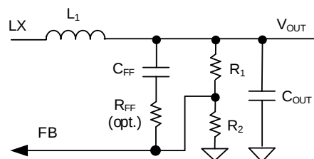
Figure 13. Feed-forward network
