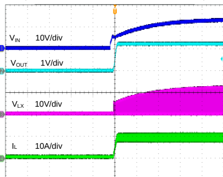
Buck Startup from V_{IN}
