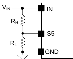
Figure 6. UVLO adjustment
