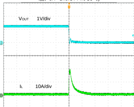
Buck Output Short Circuit ( V_{IN}=13.2V , V_{BIAS}=3.3V , V_{OUT}=1.2V , I_{OUT}=0A \sim Short, PFM, S3=0)
