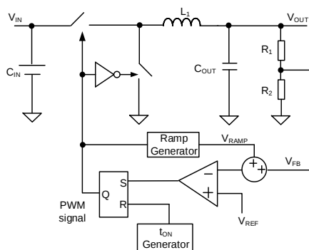
Figure 4. Instant PWM
