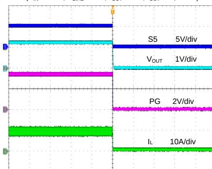
PG Test When S5 Off
