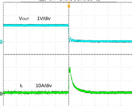
Buck Output Short Circuit ( V_{IN}=13.2V , V_{BIAS}=3.3V , V_{OUT}=1.2V , I_{OUT}=0A \sim Short, USM, S3=0)
