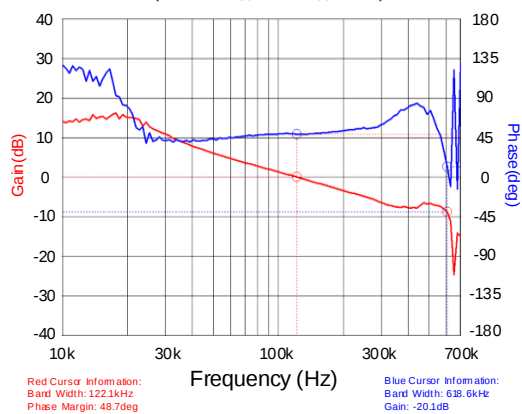
Bode Plot
