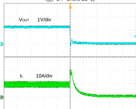
Buck Output Short Circuit ( V_{IN}=13.2V , V_{BIAS}=3.3V , V_{OUT}=1.2V , I_{OUT}=9A \sim Short, S3=0)
