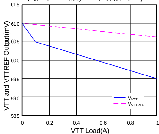
VTT Load Regulation (Source Current) ( V_{IN}=13.2V , V_{VDDQ}=1.2V , I_{VTTREF}=0mA )
