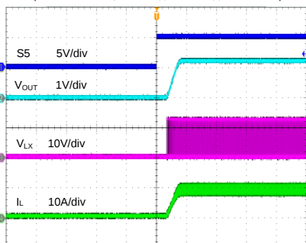
Buck Startup from S5
