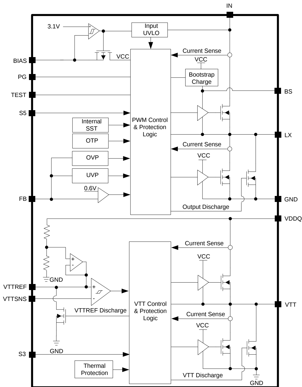
Figure 3. Block Diagram
