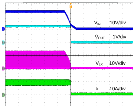
Buck Shutdown from V_{IN}
