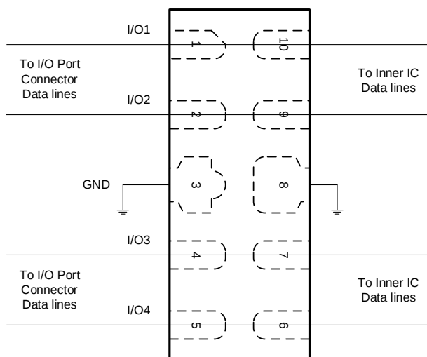
Figure 2. SY205227DVD Pin Connections in PCB
