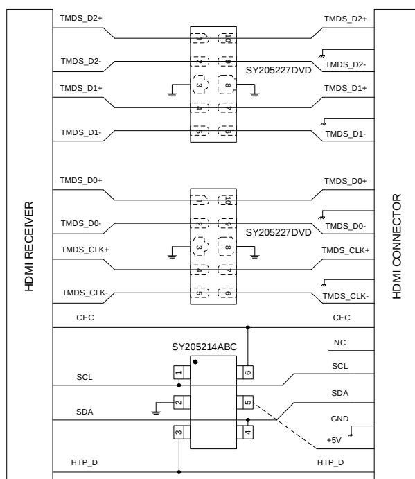
Figure 3. Layout Top View for HDMI Interface with SY205227DVD and SY205214ABC
