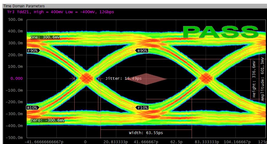
Figure 5. Data Rate 12Gb/s HDMI2.1 Eye Diagram with SY205227DVD
