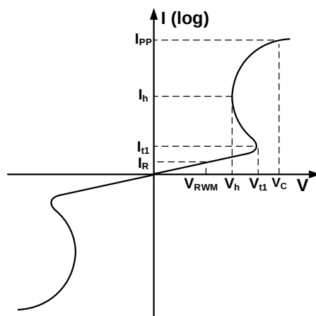
Figure 1. Bi-Directional TVS
