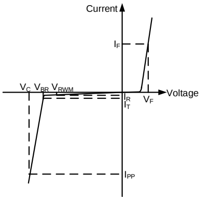
Figure 1. Uni-directional TVS
