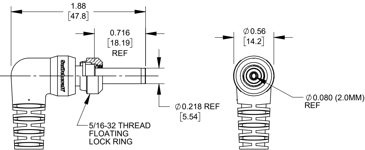
S10KS SERIES SEALED HI-AMP PLUG
