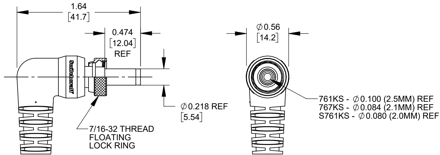
761KS, 767KS, AND S761KS SERIES SEALED PLUGS
