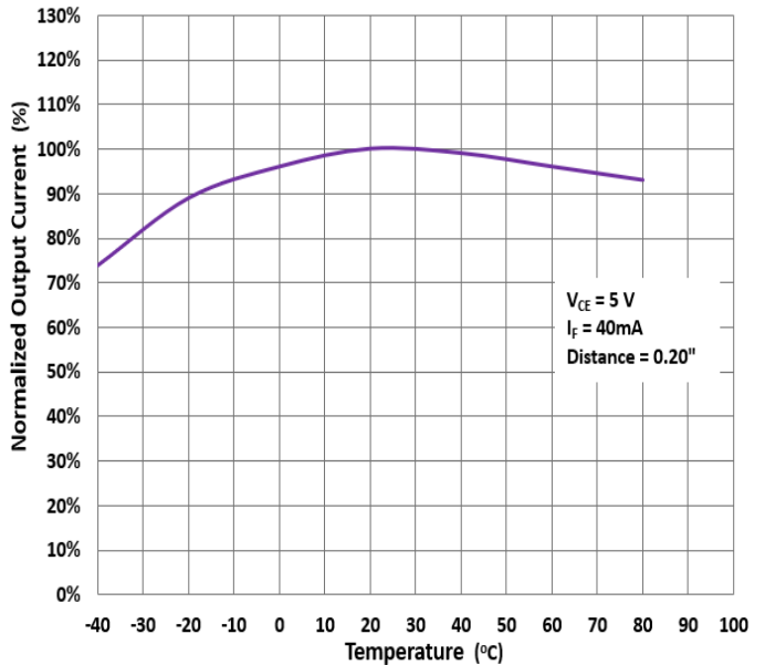
Collector Current vs Temperature
