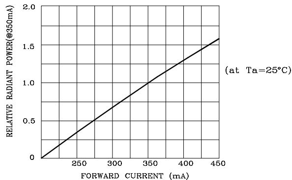
Fig.5 RELATIVE RADIANT POWER VS. FORWARD CURRENT
