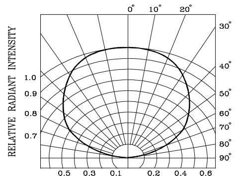
Fig.6 RADIATION DIAGRAM
