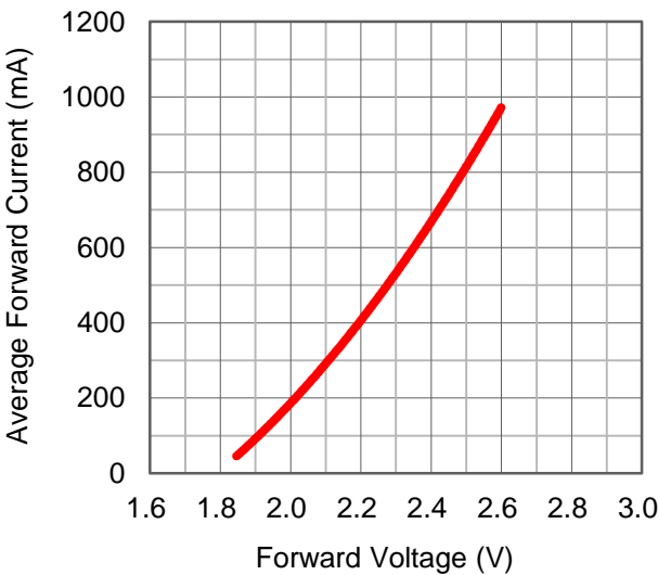
Fig 1. Forward Current vs. Forward Voltage for Red.
