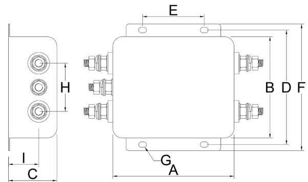
STUDS (10/15/20 AMPS)
