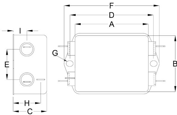
QD TABS (10/15/20 AMPS)
