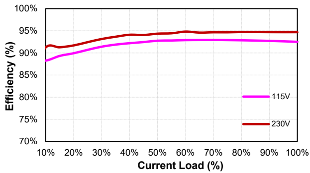
LFM420S300 (Eff Vs Io)
