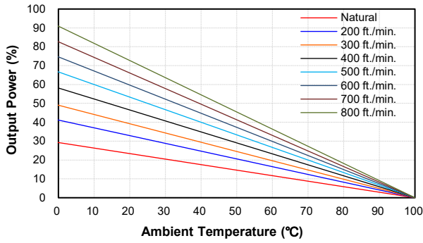
CFB600W-110S Derating Curve without Heatsink ( V_{in}=110V )
