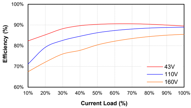
CFB600W-110S48 Eff Vs Io @25 Deg. C
