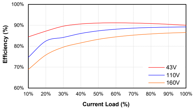
CFB600W-110S28 Eff Vs Io @25 Deg. C
