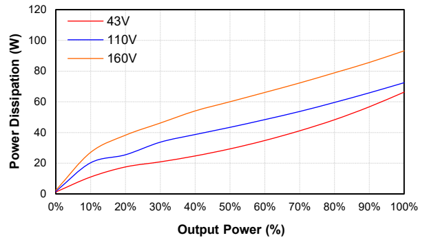
CFB600W-110S28 Pd Vs Po @25 Deg. C
