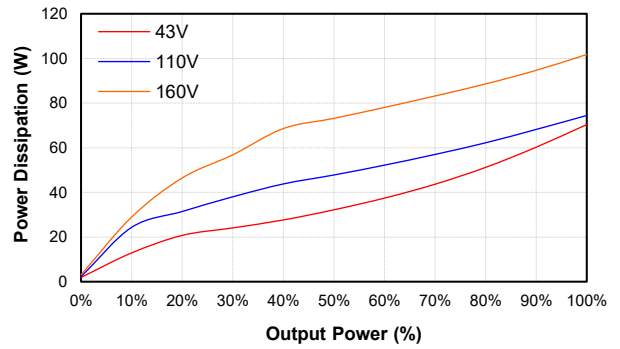
CFB600W-110S48 Pd Vs Po @25 Deg. C
