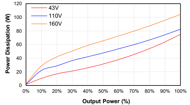
CFB600W-110S24 Pd Vs Po @25 Deg. C
