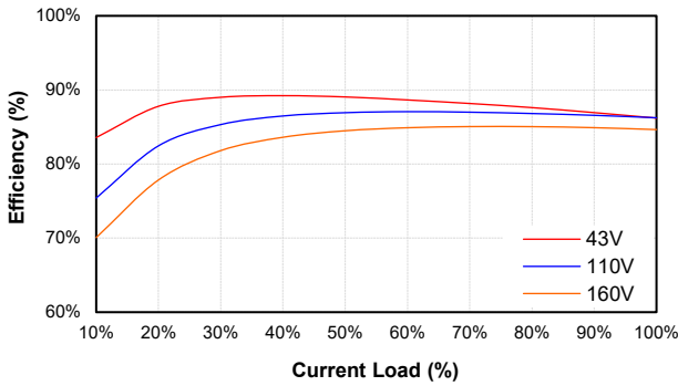
CFB600W-110S12 Eff Vs Io @25 Deg. C
