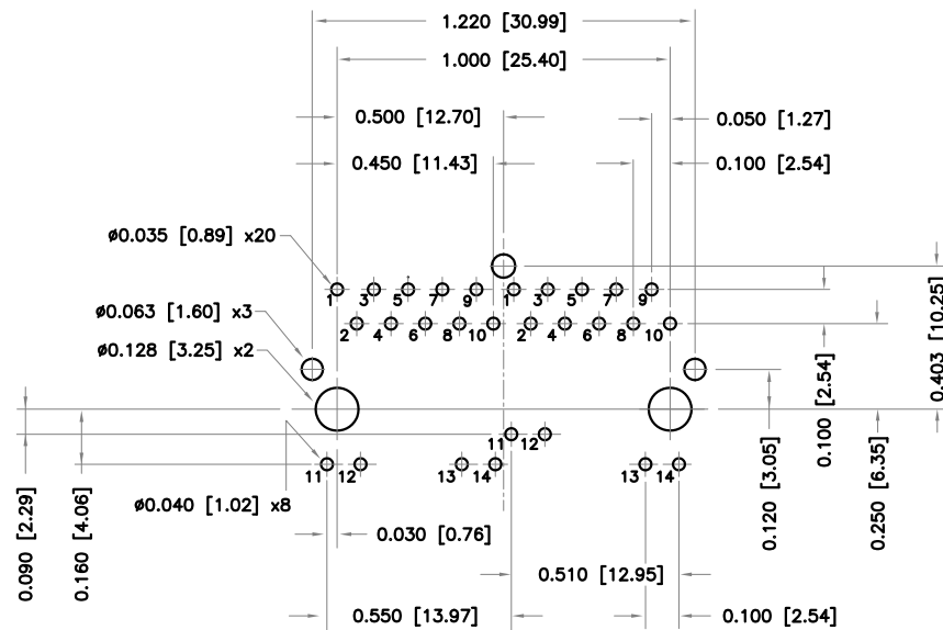
RECOMMENDED P.C. BOARD PATTERN (COMP. SIDE) DIMENSIONS: INCH [mm] TOLERANCES: \pm 0.002 [0.05] UNLESS SPECIFIED
