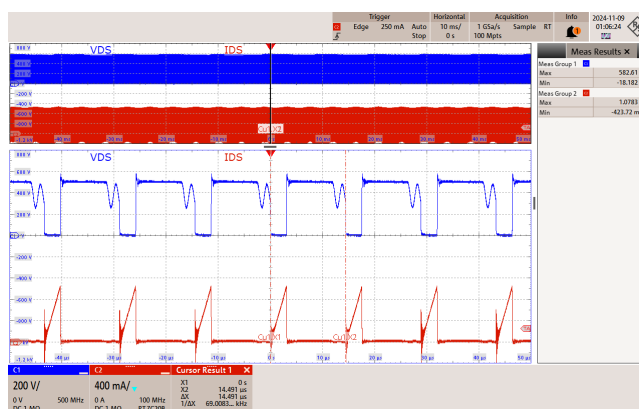
Figure 35 – 265 VAC 50 Hz.
