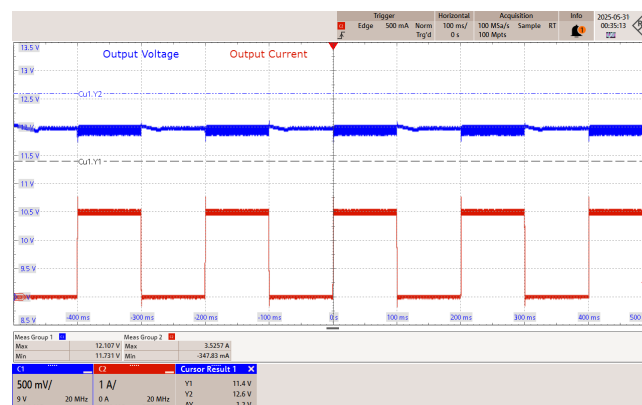
Figure 17 – 115 VAC 60 Hz.
