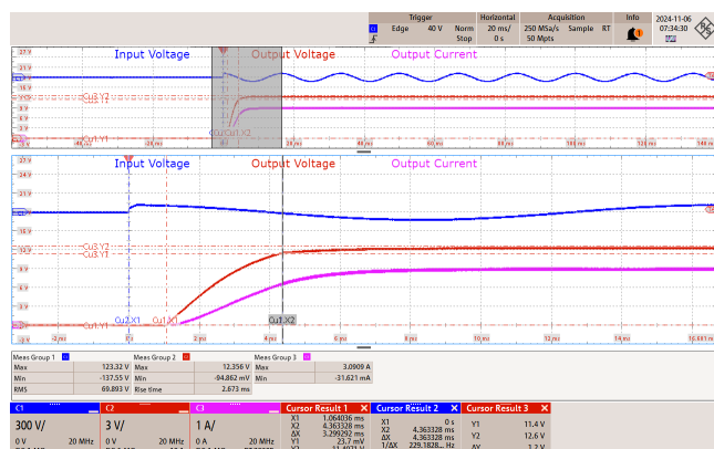
Figure 24 – 85 VAC 60 Hz.
