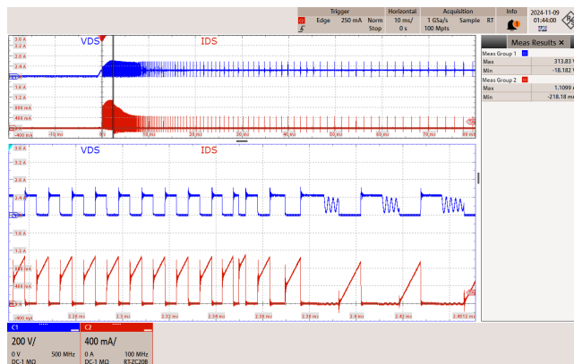
Figure 44 – 85 VAC 60 Hz.
