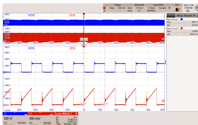
Figure 33 – 115 VAC 60 Hz.
