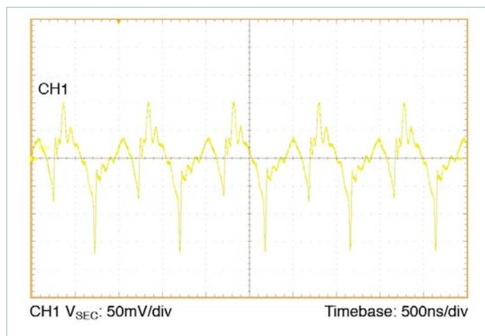
Figure 14 — Full-load secondary voltage, 10\mu\text{F } C_{PRI\_IN\_EXT} ; no external C_{SEC\_OUT\_EXT} . Board-mounted module, scope setting: 20MHz analog BW
