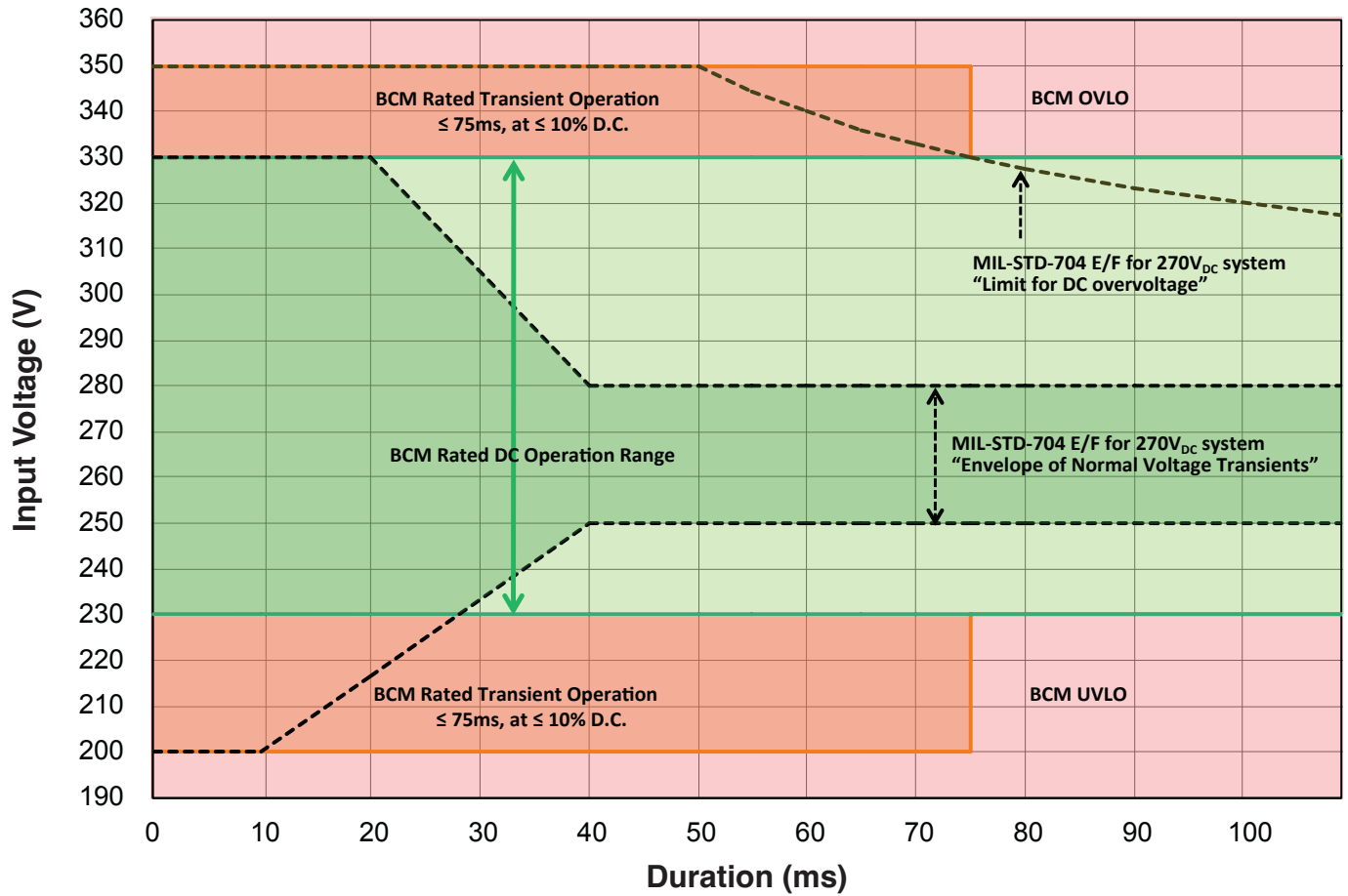
Figure 19 — Envelope of normal voltage transient for 270\text{V}_{\text{DC}} system.
