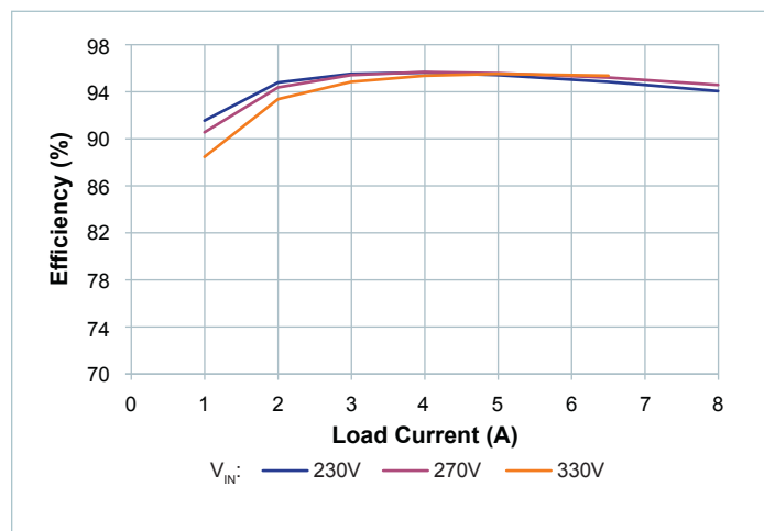
Figure 9 — Efficiency at T_{CASE} = 85^{\circ}\text{C}
