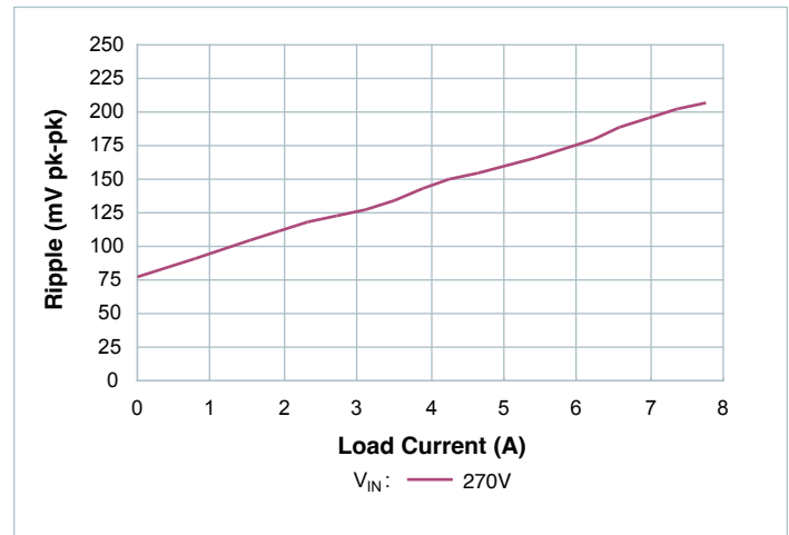
Figure 14 — V_{RIPPLE} vs. I_{OUT} ; no external C_{OUT} ; board-mounted module, scope setting: 20MHz analog BW
