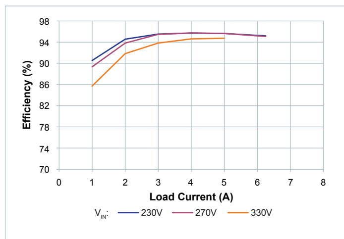
Figure 11 — Efficiency at T_{CASE} = 100^{\circ}\text{C}
