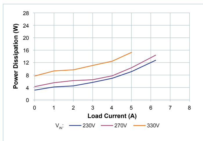
Figure 12 — Power dissipation at T_{CASE} = 100^{\circ}\text{C}
