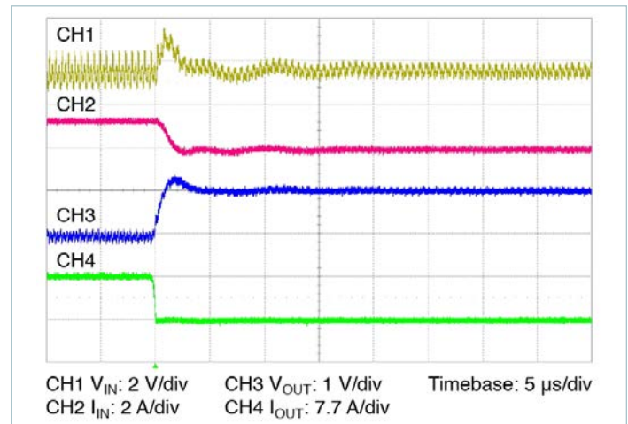
Figure 18 — 8.00 – 0A transient response: C_{IN} = 100\mu\text{F} , no external C_{OUT}
