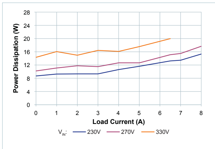
Figure 6 — Power dissipation at T_{CASE} = -55^{\circ}\text{C}
