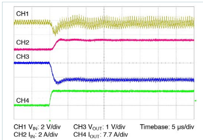
Figure 17 — 0 – 8.00A transient response: C_{IN} = 100\mu\text{F} , no external C_{OUT}
