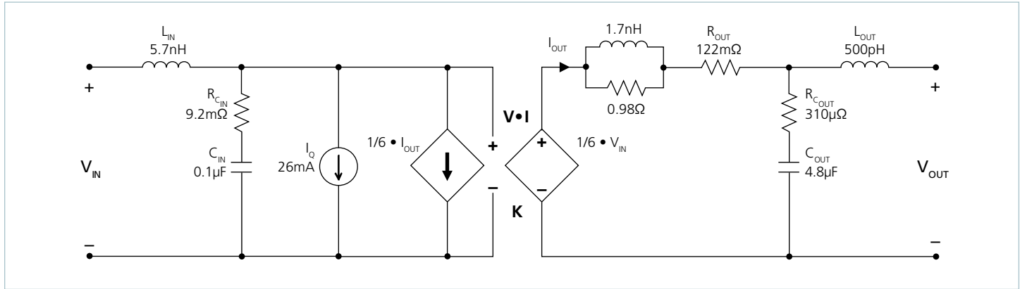
Figure 20 — VI Chip® module AC model
