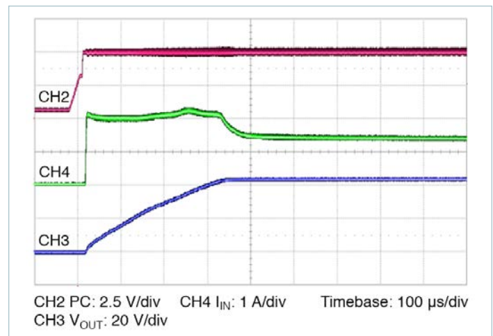
Figure 16 — Start up from application of PC; V_{IN} pre-applied C_{OUT} = 50\mu\text{F}
