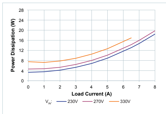
Figure 10 — Power dissipation at T_{CASE} = 85^{\circ}\text{C}
