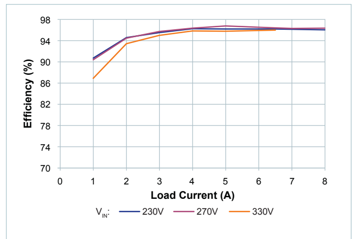
Figure 7 — Efficiency at T_{CASE} = 25^{\circ}\text{C}
