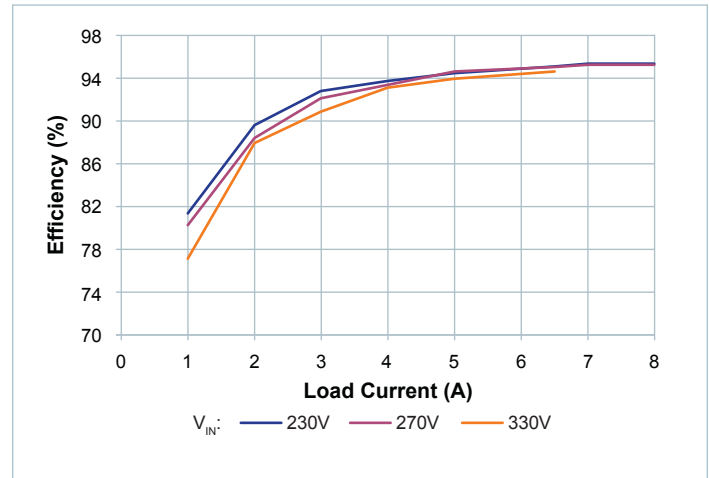
Figure 5 — Efficiency at T_{CASE} = -55^{\circ}\text{C}
