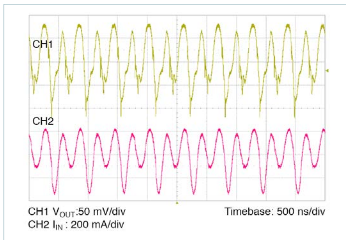
Figure 15 — Full-load ripple, 100\mu\text{F } C_{IN} ; no external C_{OUT} ; board-mounted module, scope setting: 20MHz analog BW
