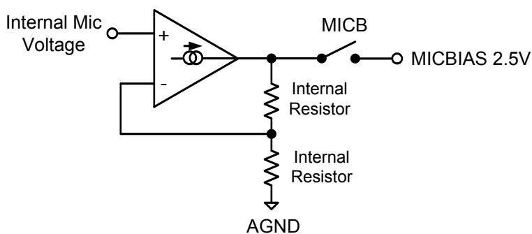
Figure 17. Mic Bias
