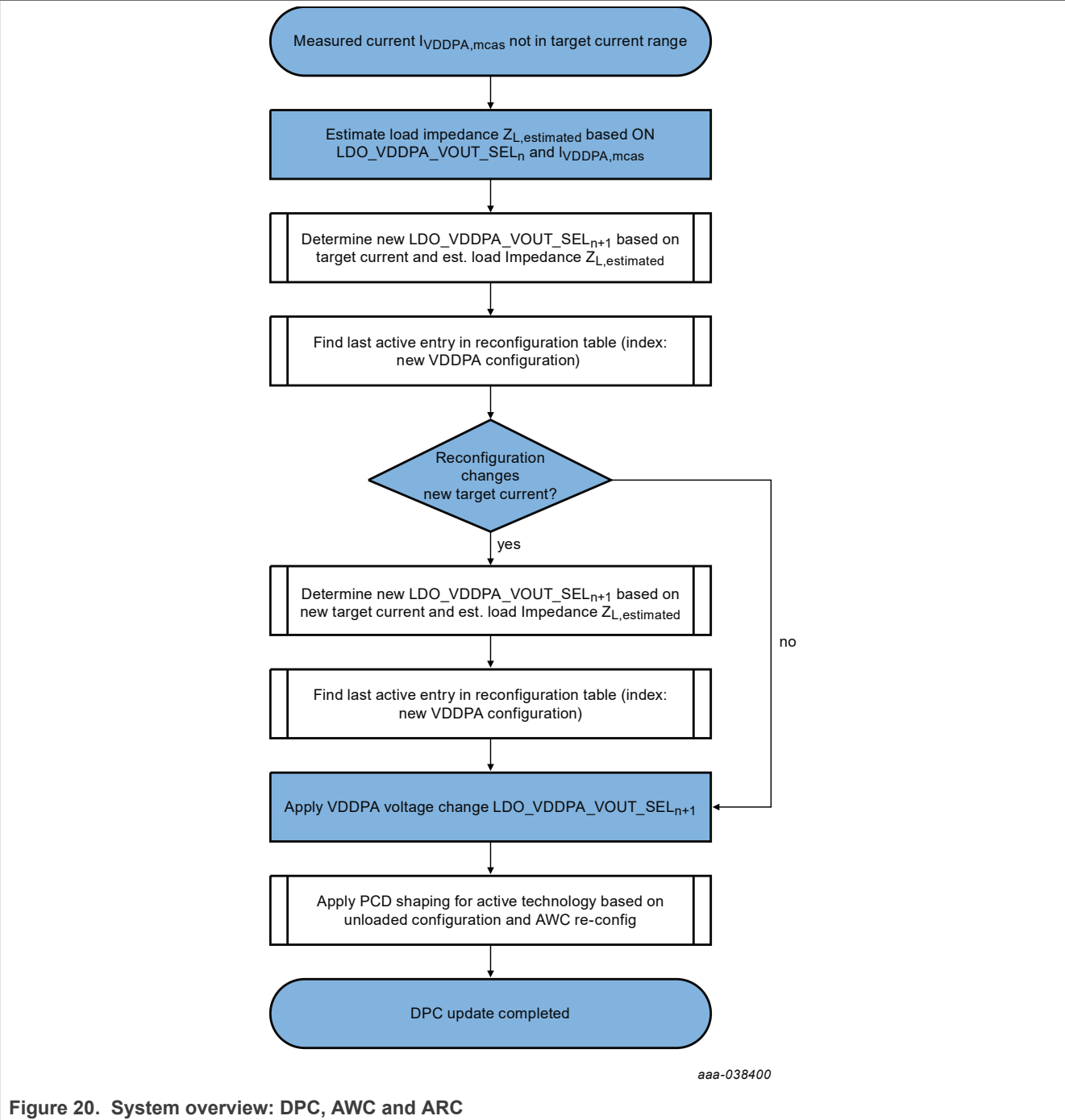
Figure 20. System overview: DPC, AWC and ARC
