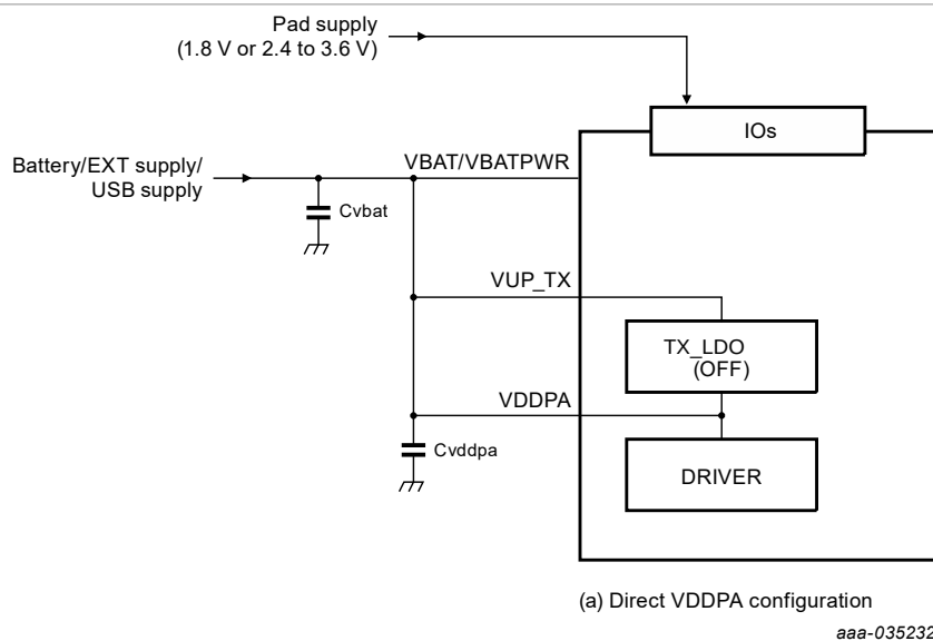
Figure 7. Direct transmitter supply
