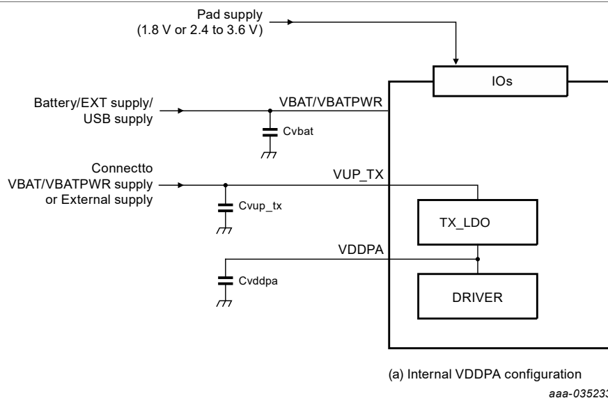
Figure 6. Transmitter supply
