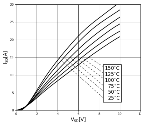
Figure 12. Forward Characteristics of Rev. Diode
