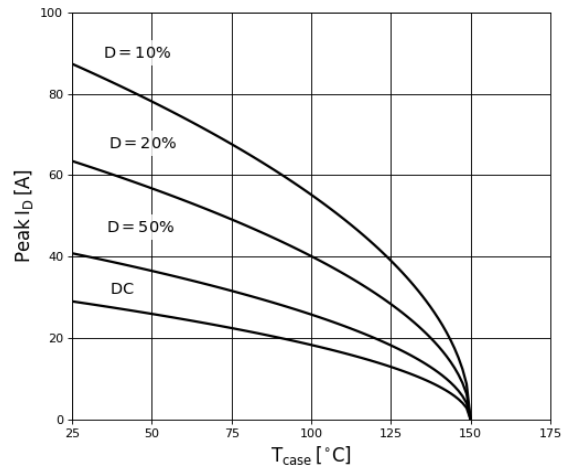
Figure 11. Current Derating
