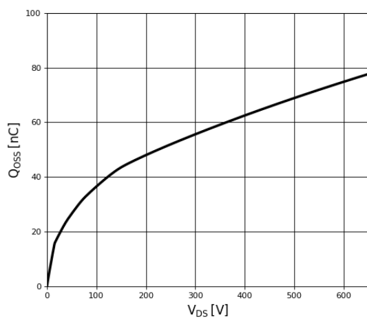
Figure 8. Typical Q_{oss}
