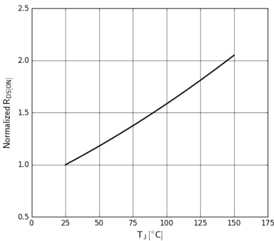
Figure 5. Normalized On-resistance I_D = 18\text{A} , V_{GS} = 12\text{V}
