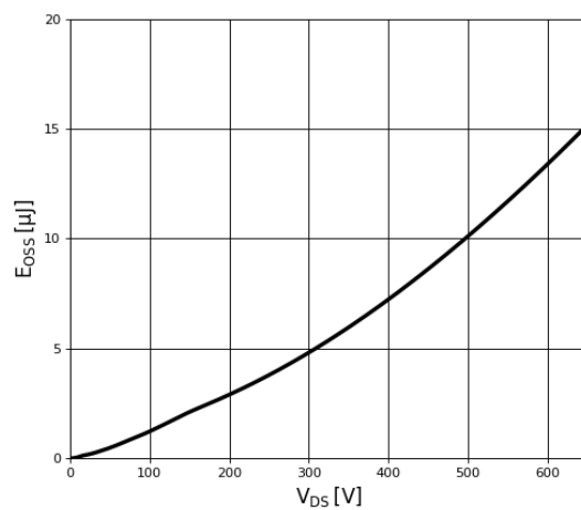
Figure 7. Typical C_{oss} Stored Energy
