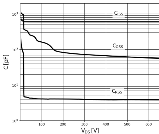
Figure 6. Typical Capacitance
