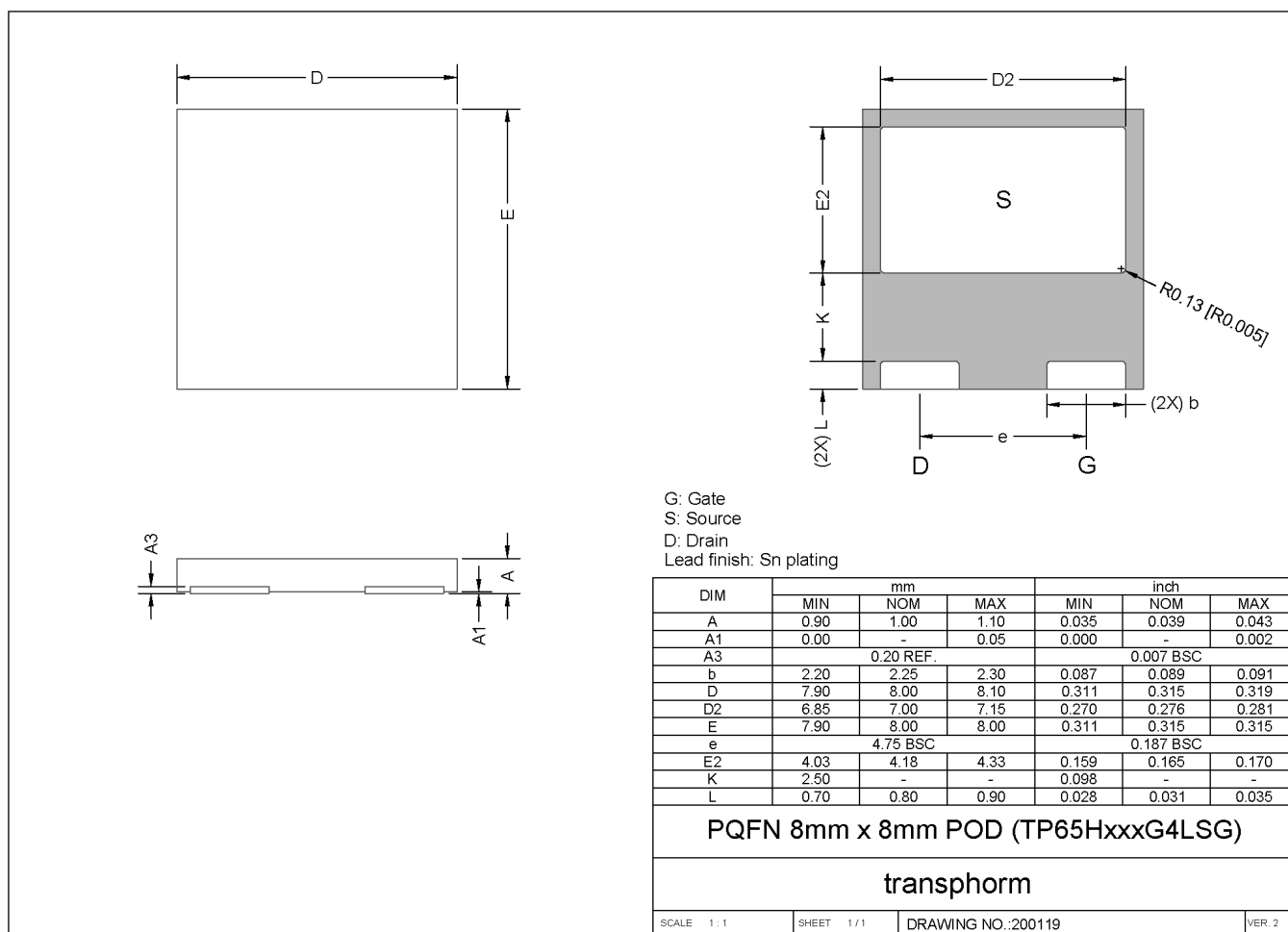
Figure 19. 8 × 8 mm PQFN Package Outline Drawing
