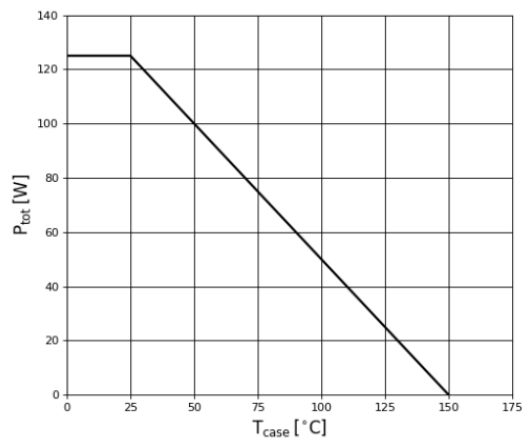
Figure 10. Power Dissipation
