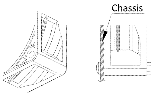
● RIB TYPE FIGURE 2
