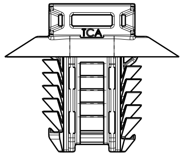
Mount Delivery condition: unassembled set
